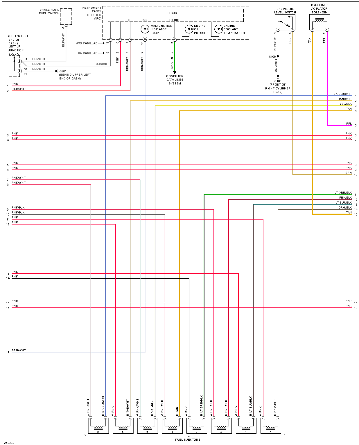
Fig. 27: 6.2L VIN 8, Engine Performance Circuit (3 of 5)
