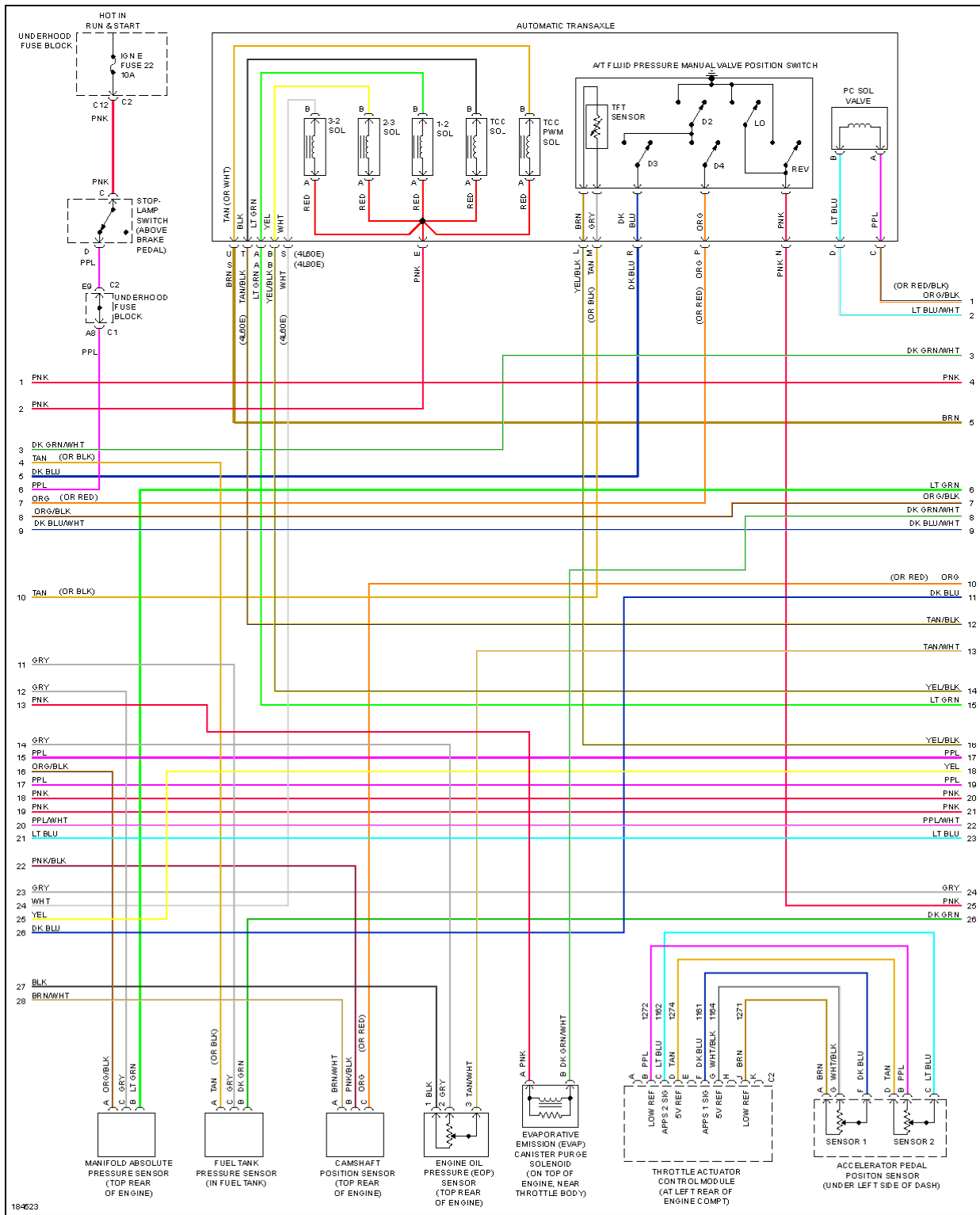
Fig. 39: 6.0L VIN U, Engine Performance Circuit (3 of 5)
