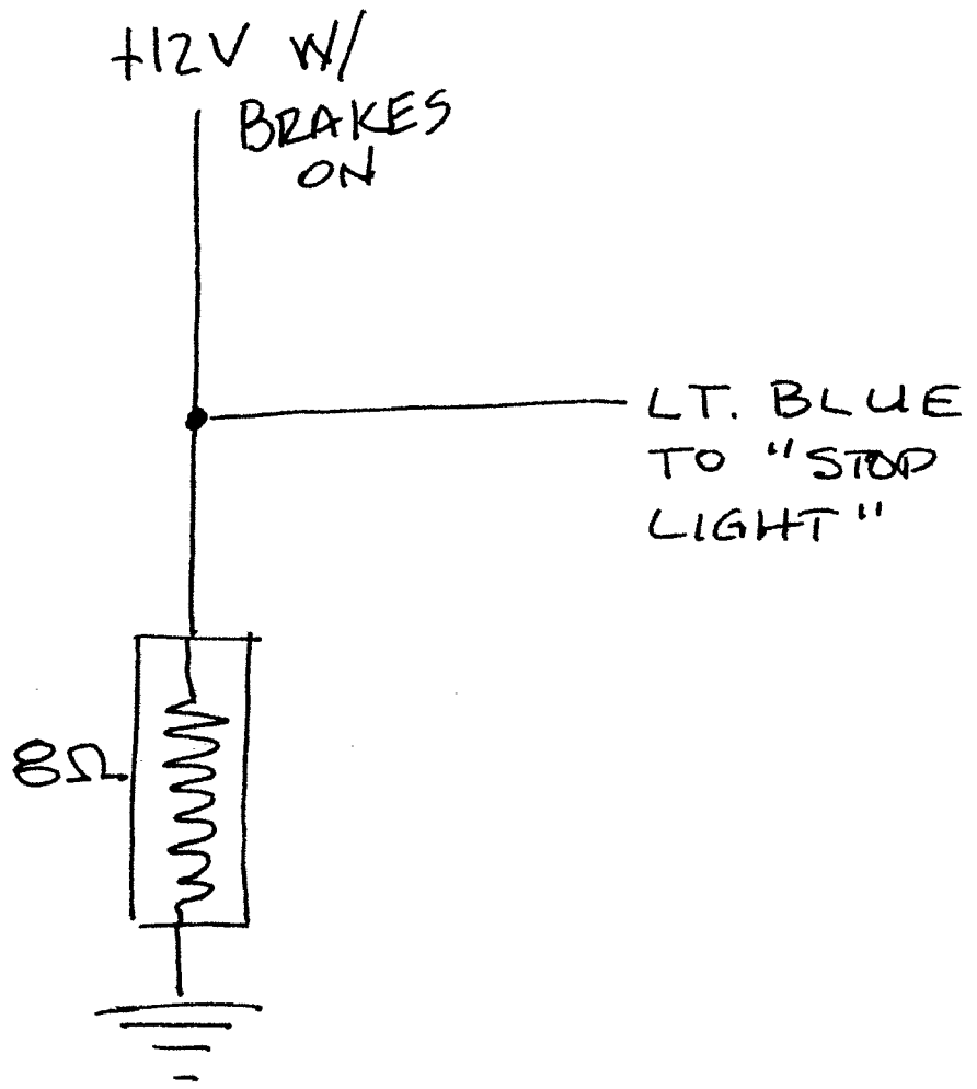
STOP LAMP WIRING DBW CRUISE CONTROL
