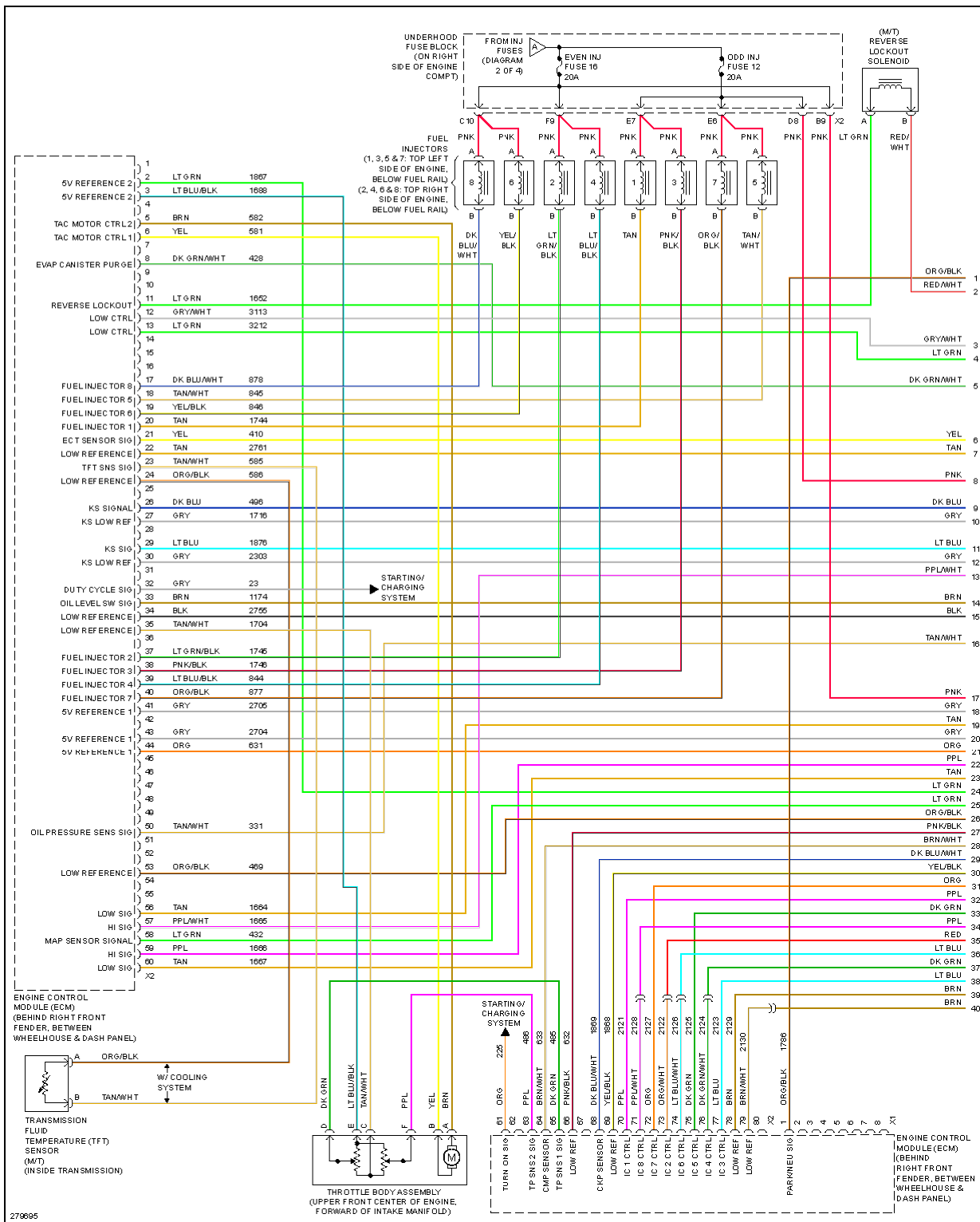
Fig. 22: 6.2L VIN W, Engine Performance Circuit (1 of 4)
