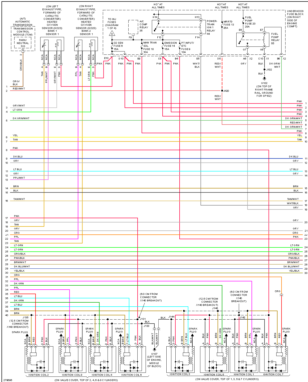
Fig. 23: 6.2L VIN W, Engine Performance Circuit (2 of 4)
