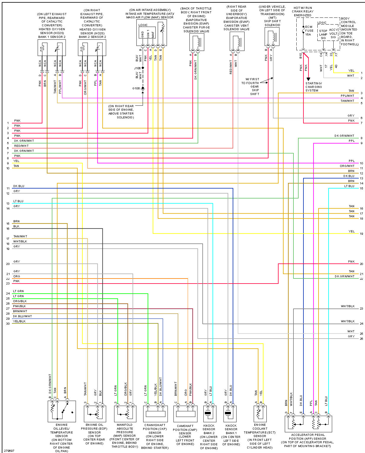
Fig. 24: 6.2L VIN W, Engine Performance Circuit (3 of 4)
