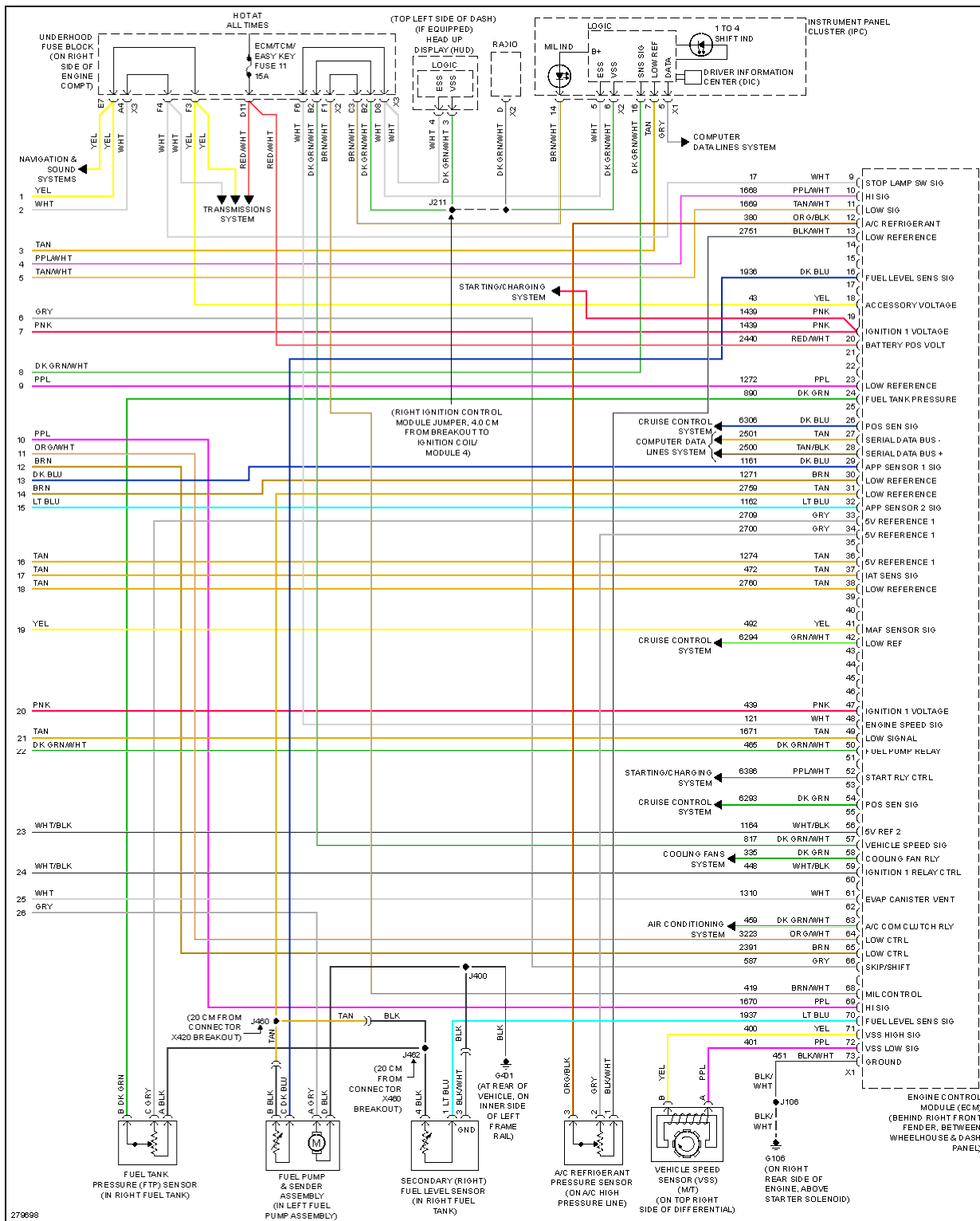
Fig. 25: 6.2L VIN W, Engine Performance Circuit (4 of 4)
