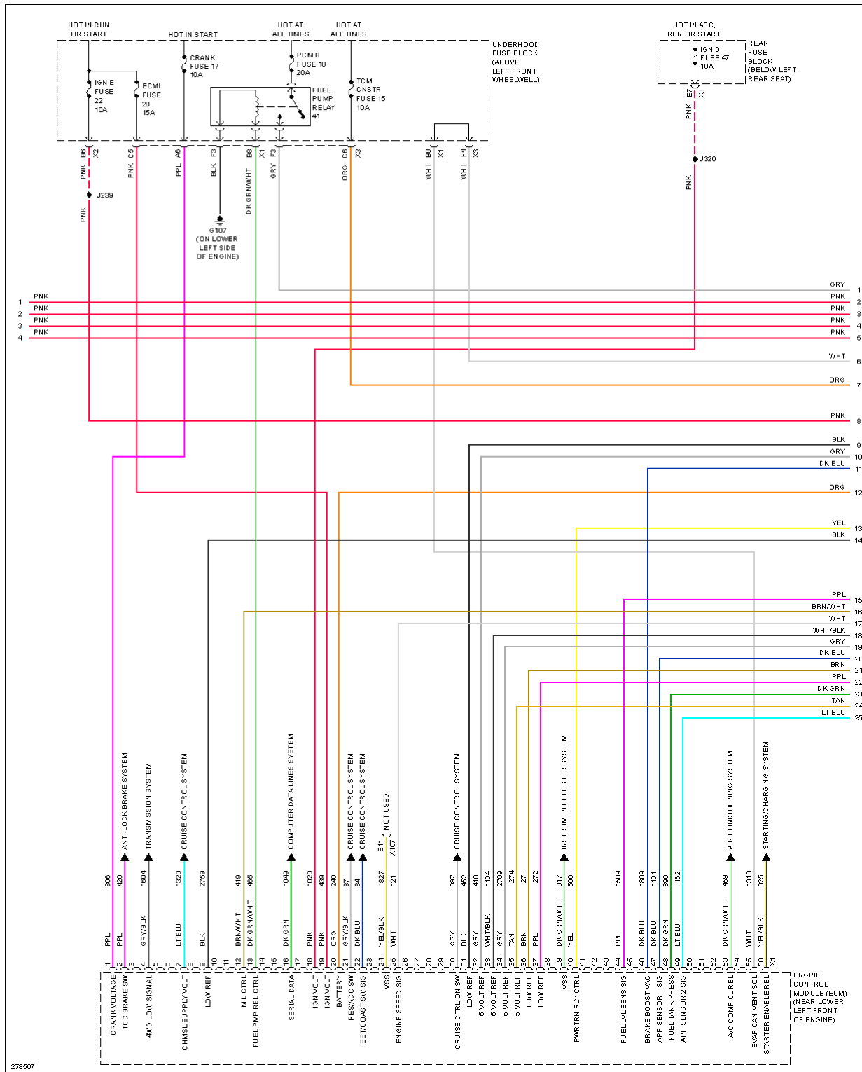
Fig. 28: 6.0L VIN H, Engine Performance Circuit (2 of 5)
