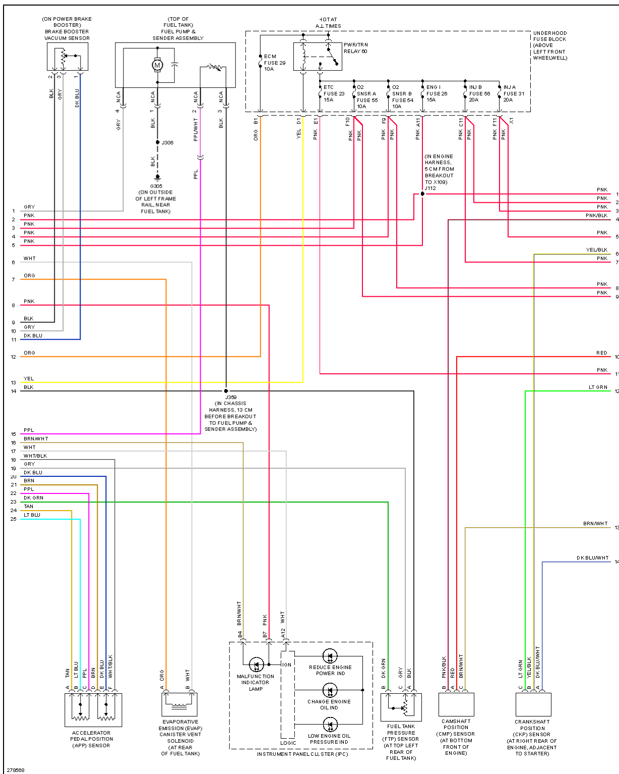
Fig. 29: 6.0L VIN H, Engine Performance Circuit (3 of 5)
