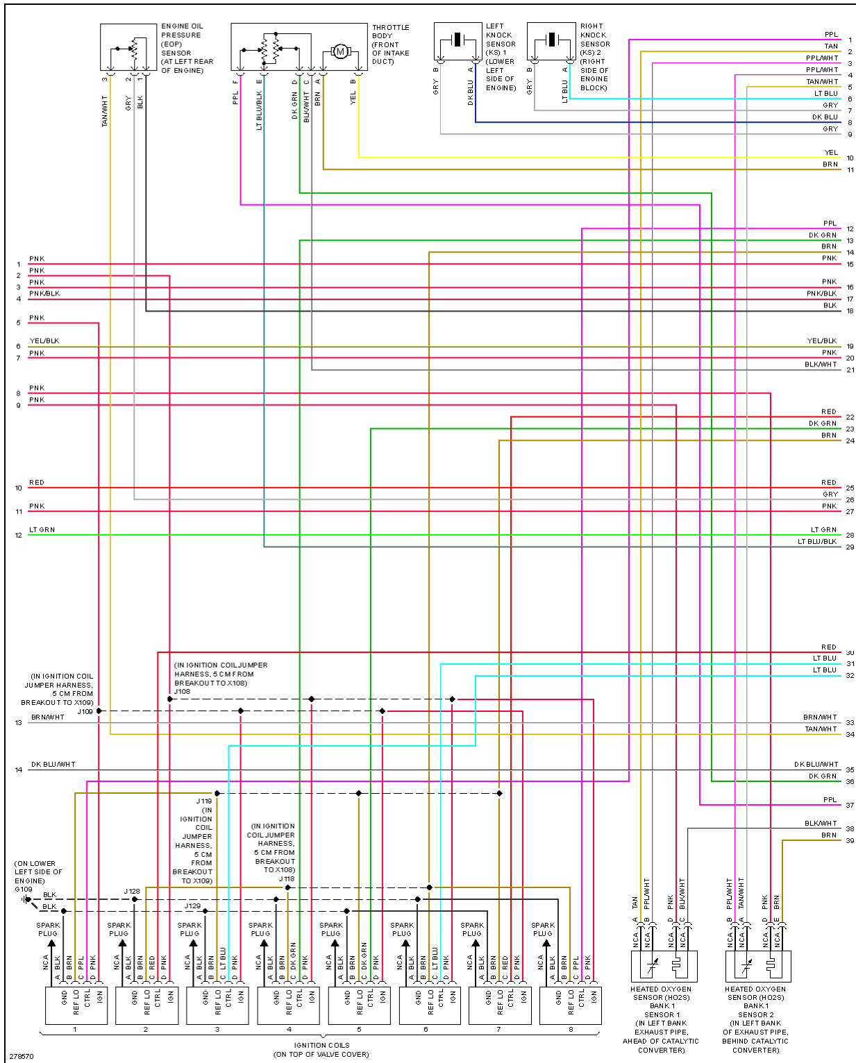
Fig. 30: 6.0L VIN H, Engine Performance Circuit (4 of 5)
