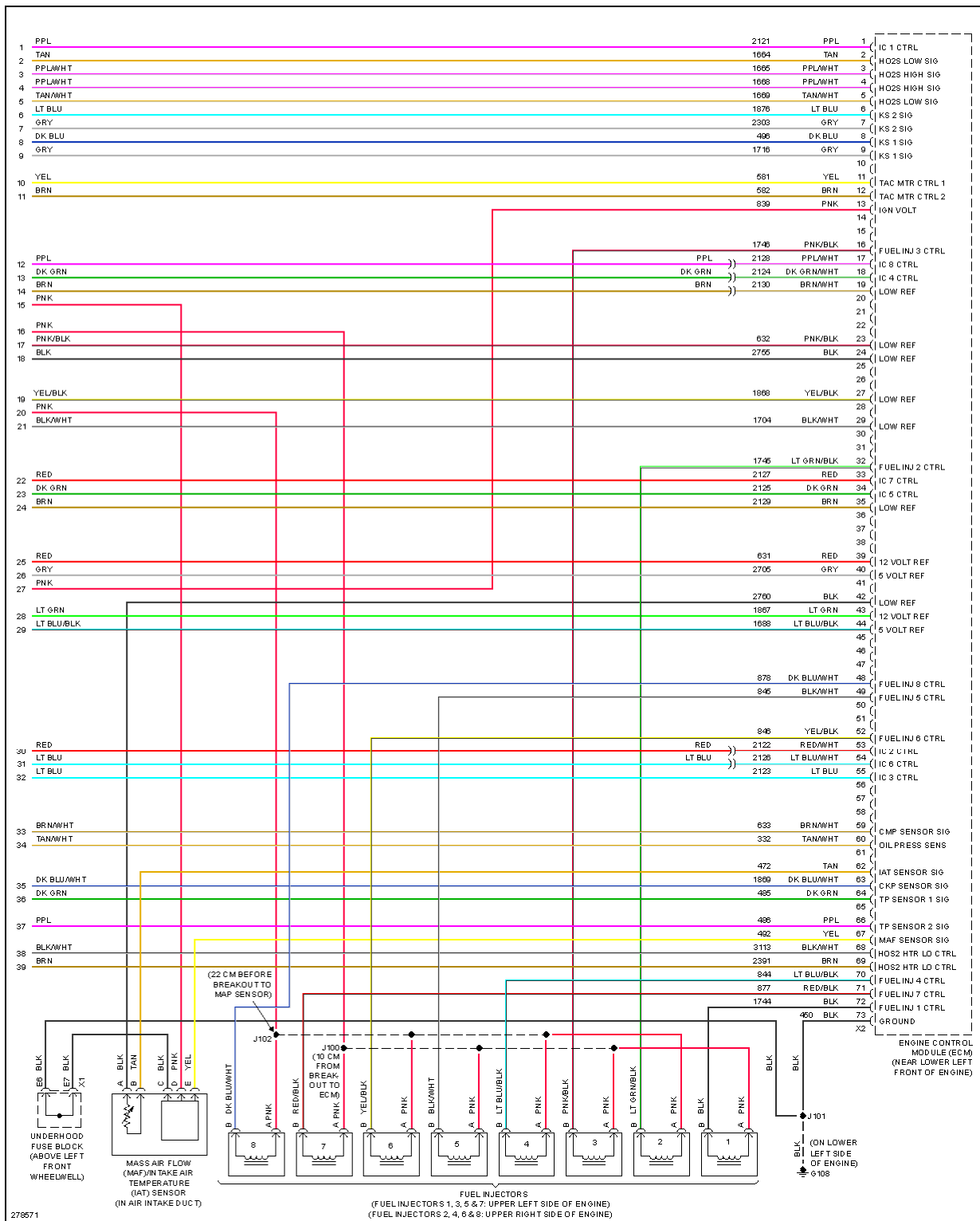
Fig. 31: 6.0L VIN H, Engine Performance Circuit (5 of 5)
