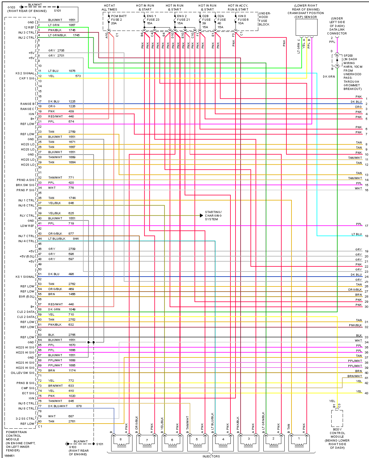
Fig. 14: 6.0L VIN U, Engine Performance Circuit (1 of 5)
