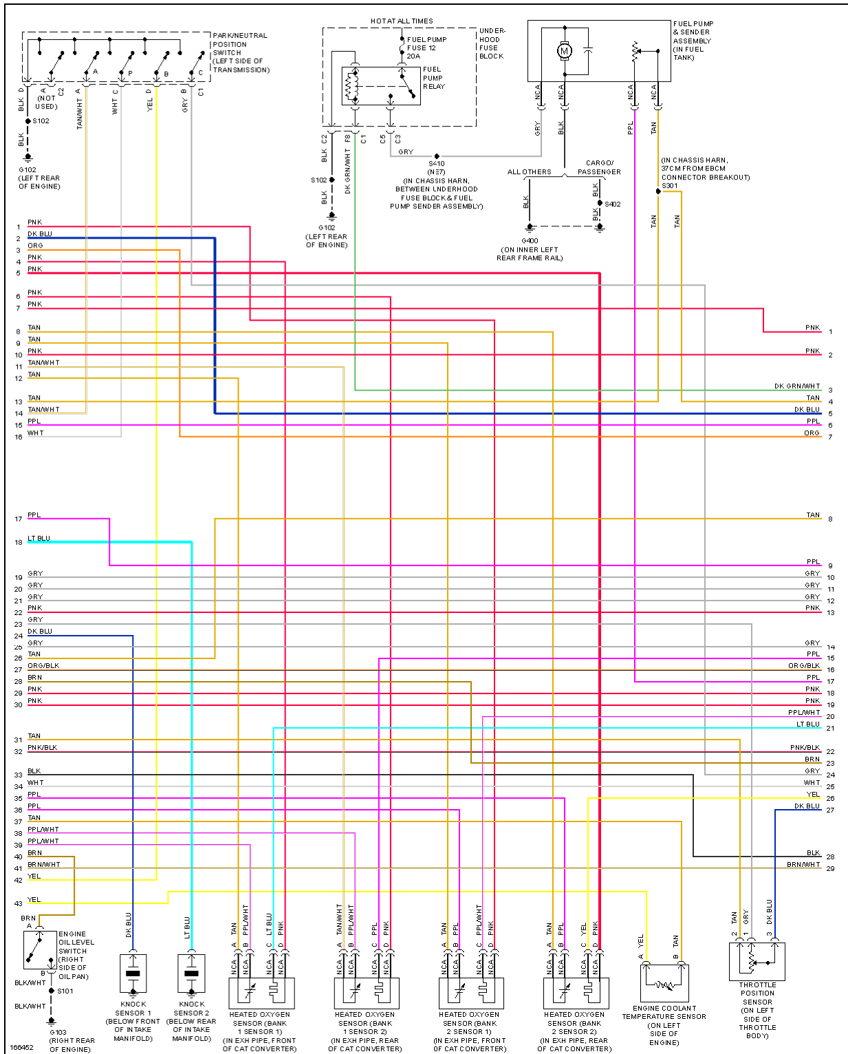
Fig. 15: 6.0L VIN U, Engine Performance Circuit (2 of 5)
