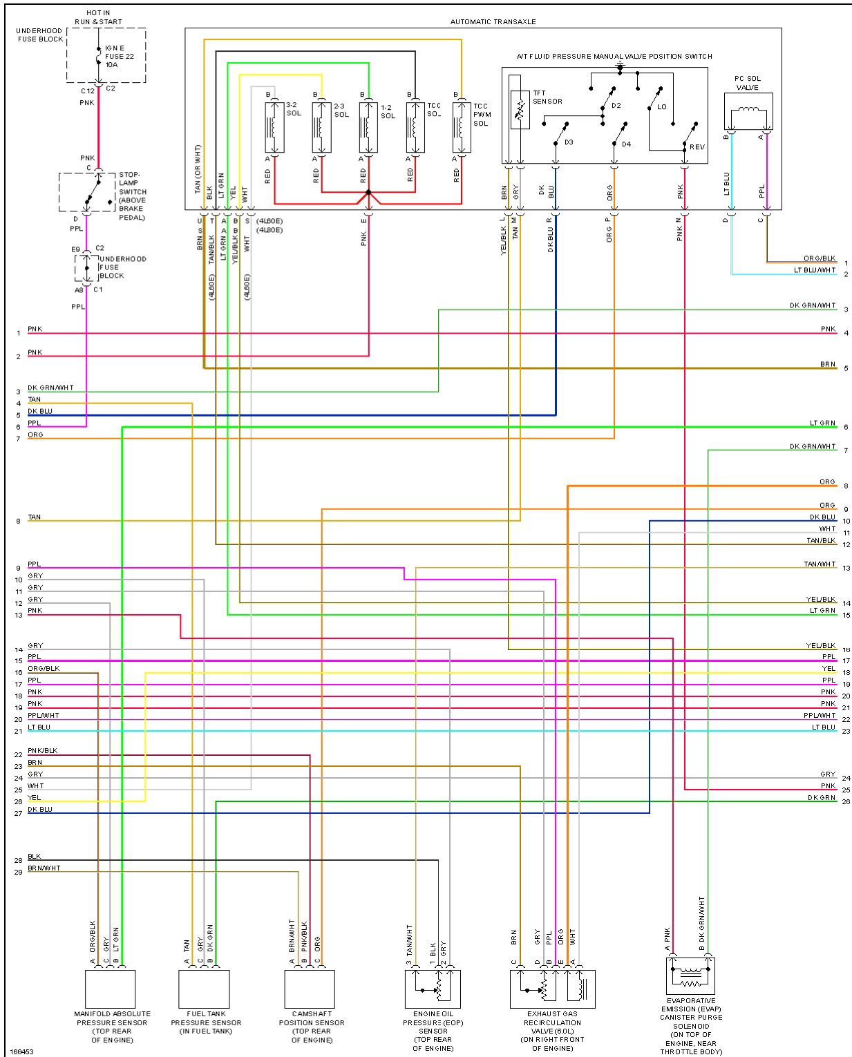
Fig. 16: 6.0L VIN U, Engine Performance Circuit (3 of 5)
