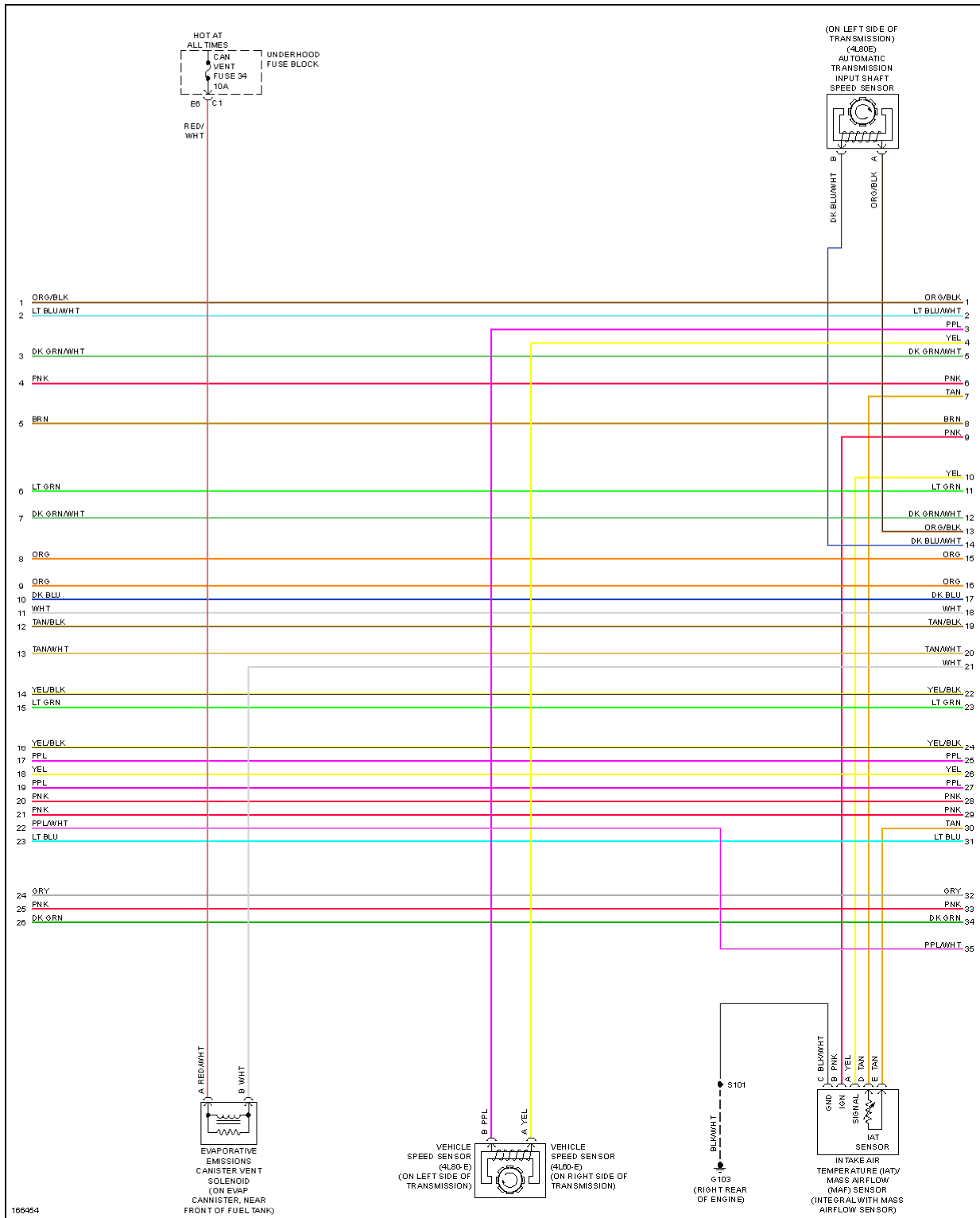
Fig. 17: 6.0L VIN U, Engine Performance Circuit (4 of 5)
