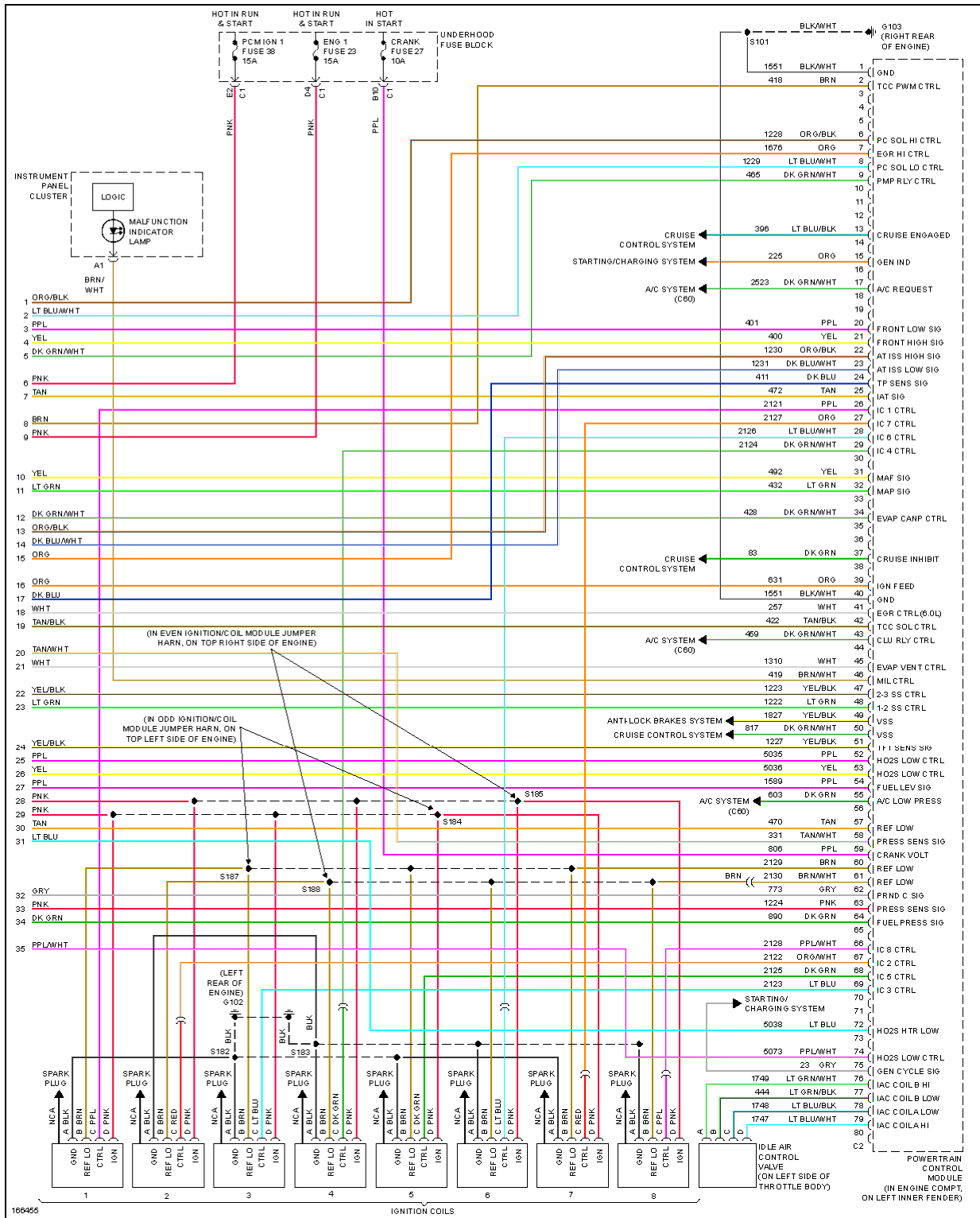
Fig. 18: 6.0L VIN U, Engine Performance Circuit (5 of 5)
