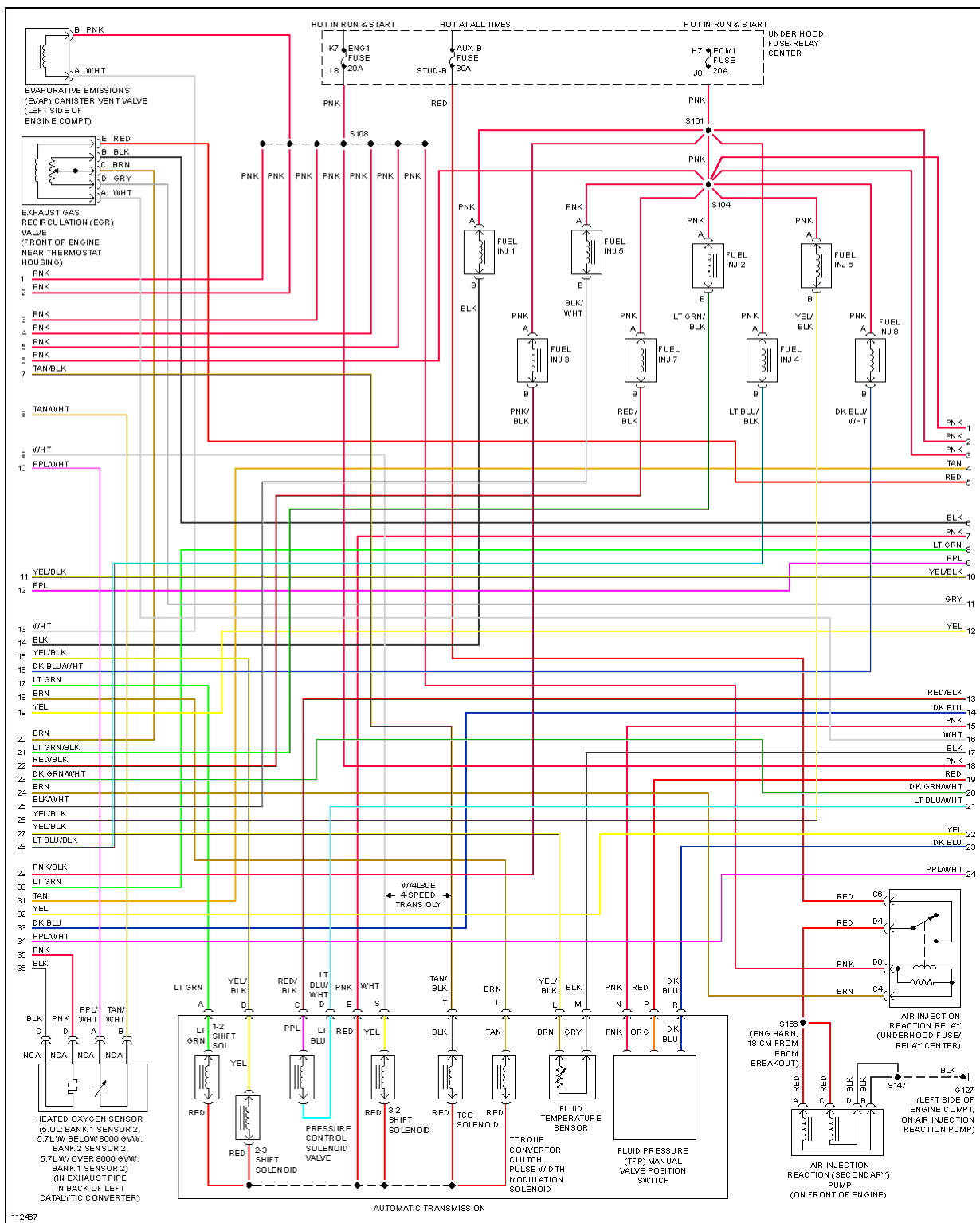
Fig. 17: 5.7L VIN R, Engine Performance Circuits (2 of 4)
