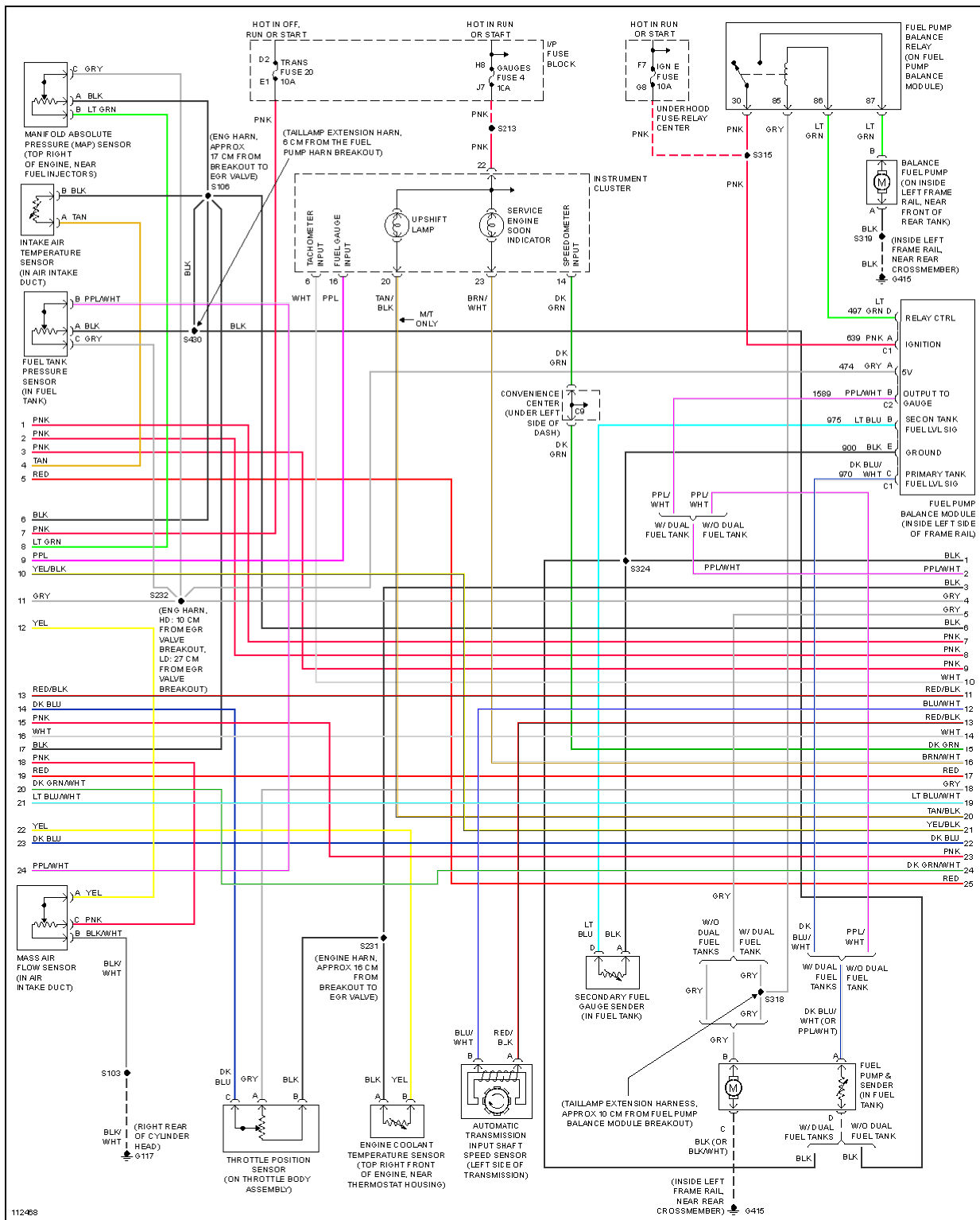
Fig. 18: 5.7L VIN R, Engine Performance Circuits (3 of 4)
