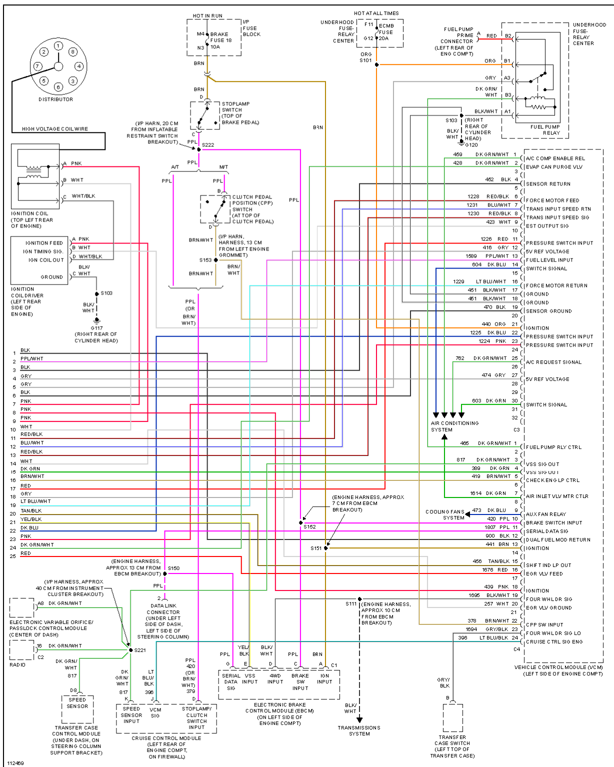
Fig. 19: 5.7L VIN R, Engine Performance Circuits (4 of 4)
