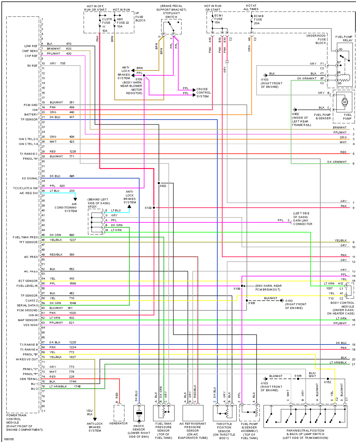
Fig. 13: 2.2L VIN 5, Engine Performance Circuit (1 of 3)
