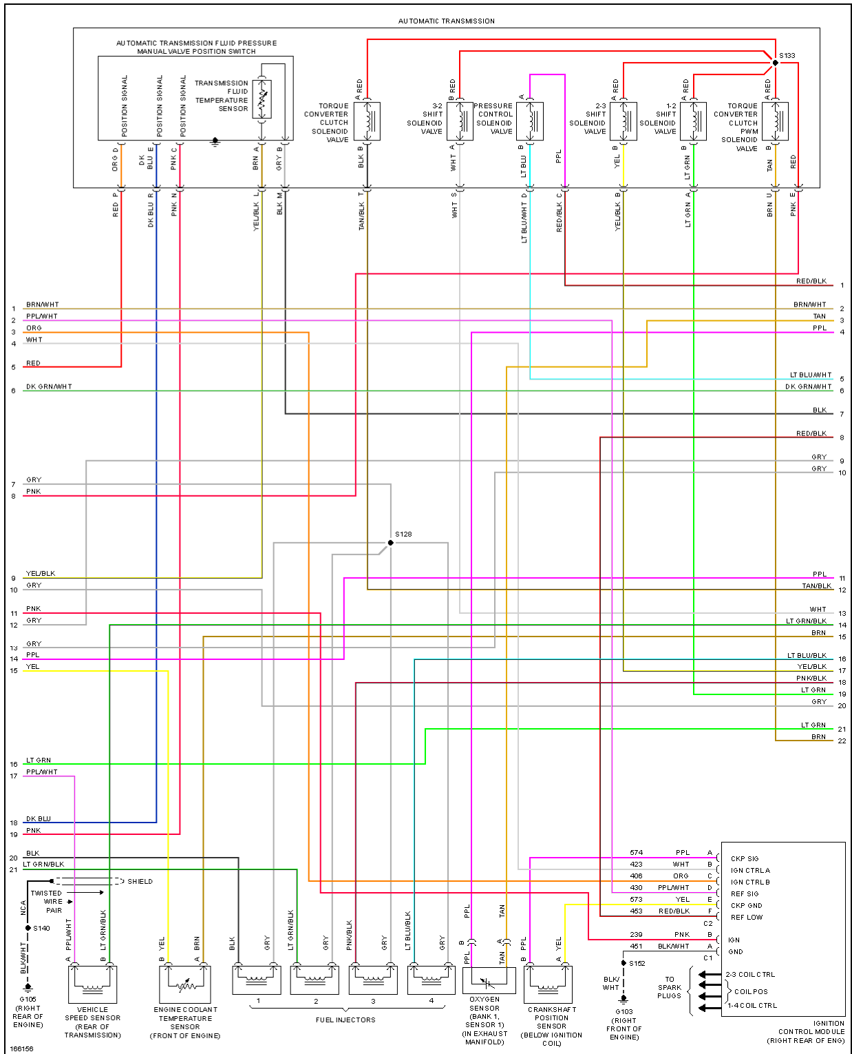
Fig. 14: 2.2L VIN 5, Engine Performance Circuit (2 of 3)
