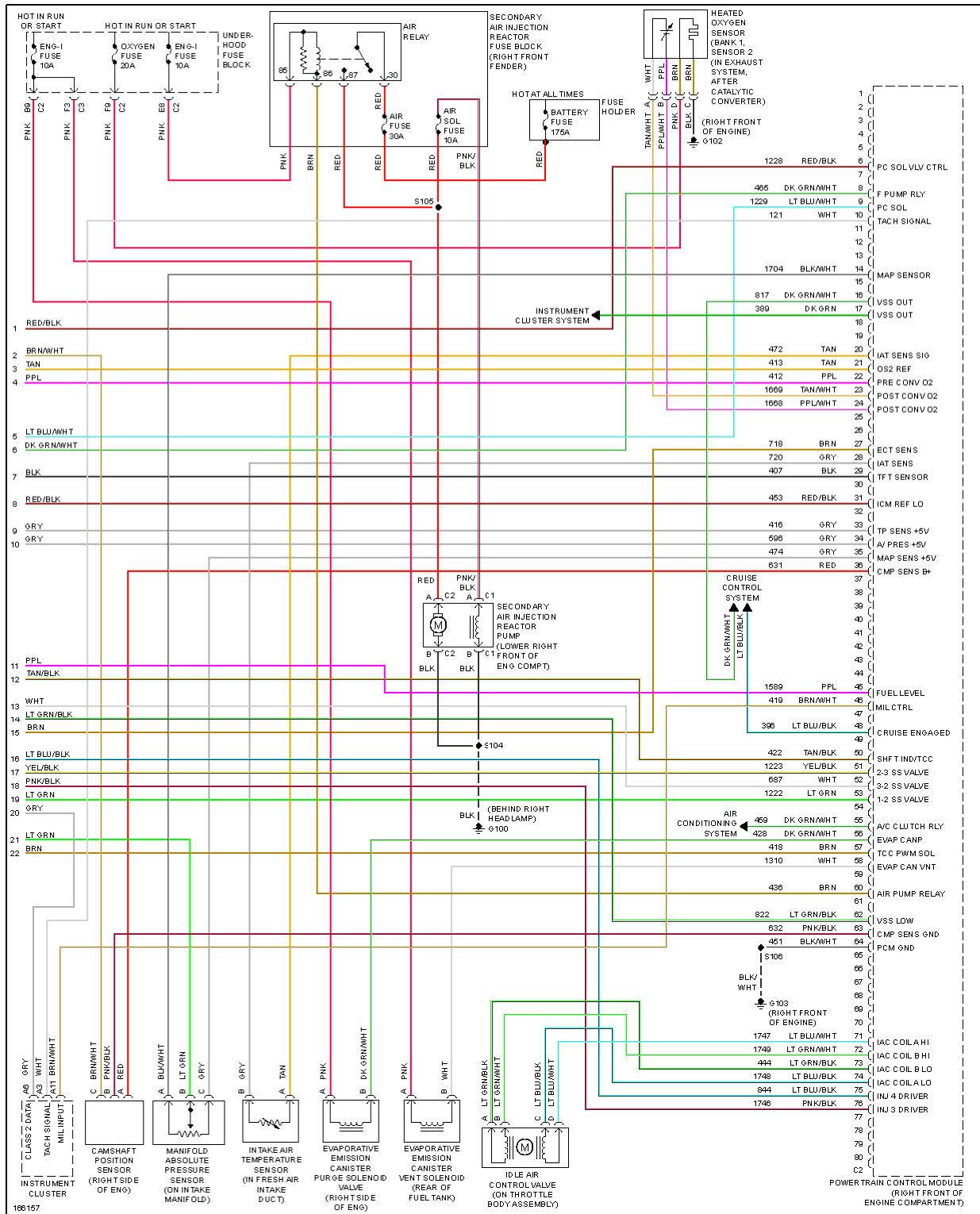
Fig. 15: 2.2L VIN 5, Engine Performance Circuit (3 of 3)
