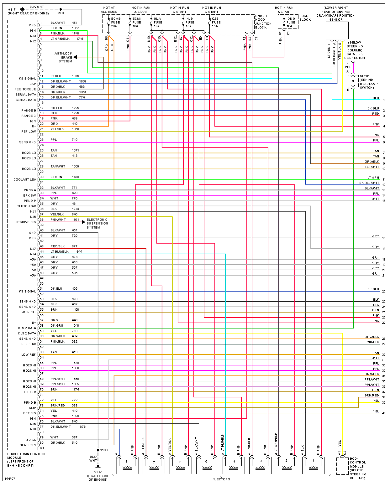
Fig. 16: 6.0L VIN U, Engine Performance Circuits (1 of 5)
