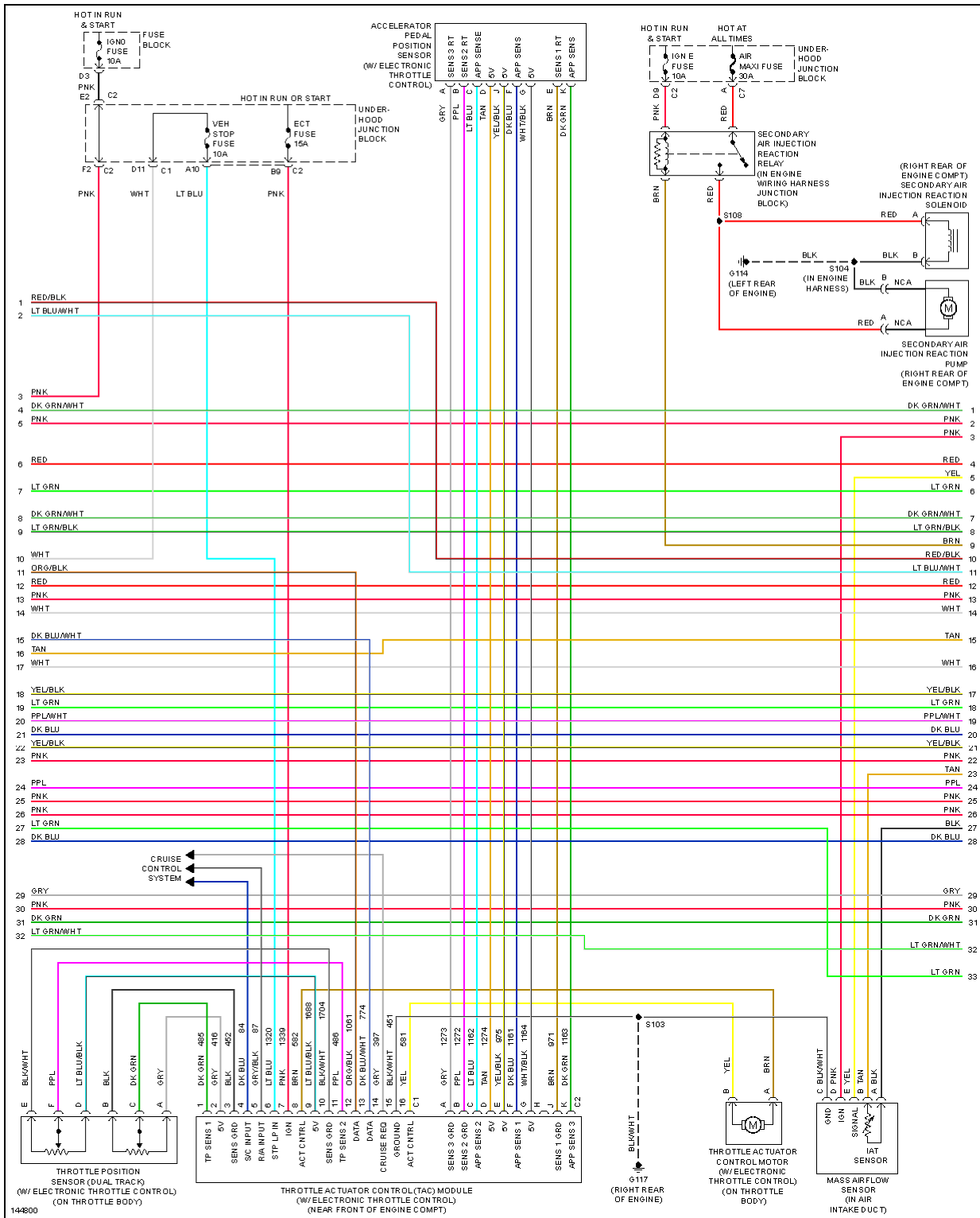
Fig. 19: 6.0L VIN U, Engine Performance Circuits (4 of 5)
