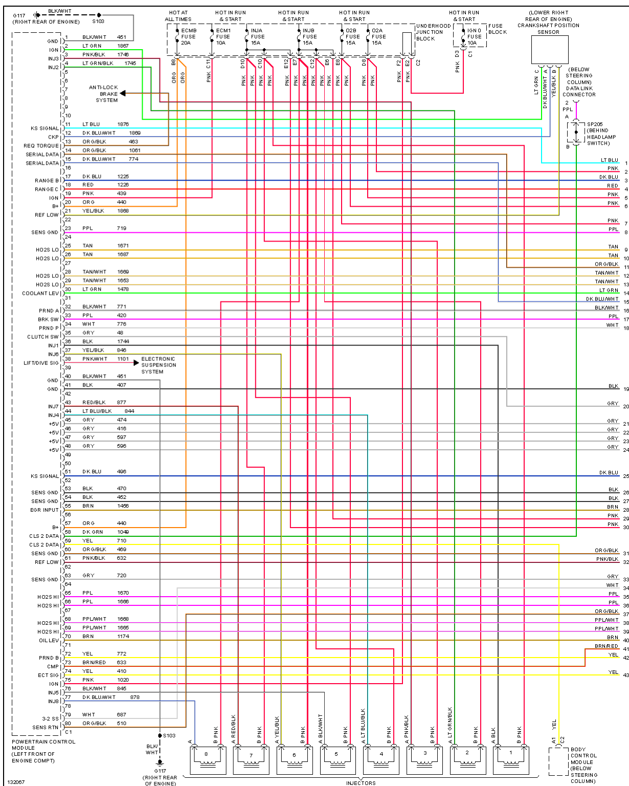
Fig. 33: 5.3L VIN T, Engine Performance Circuits, W/ Delphi HO2S (1 of 5)
