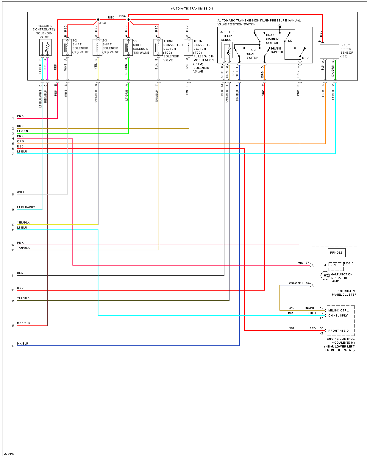
Fig. 77: A/T Circuit (2 of 2)
