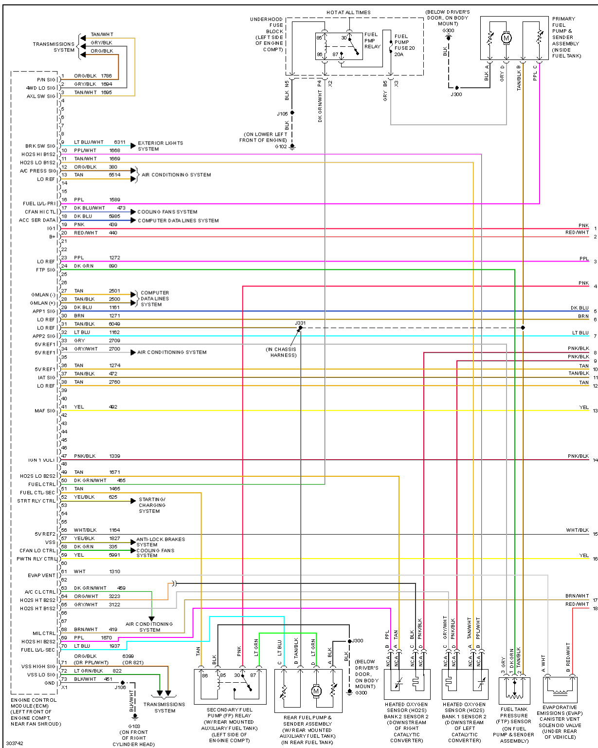
Fig. 24: 6.0L VIN K, Engine Performance Circuit (1 of 5)
