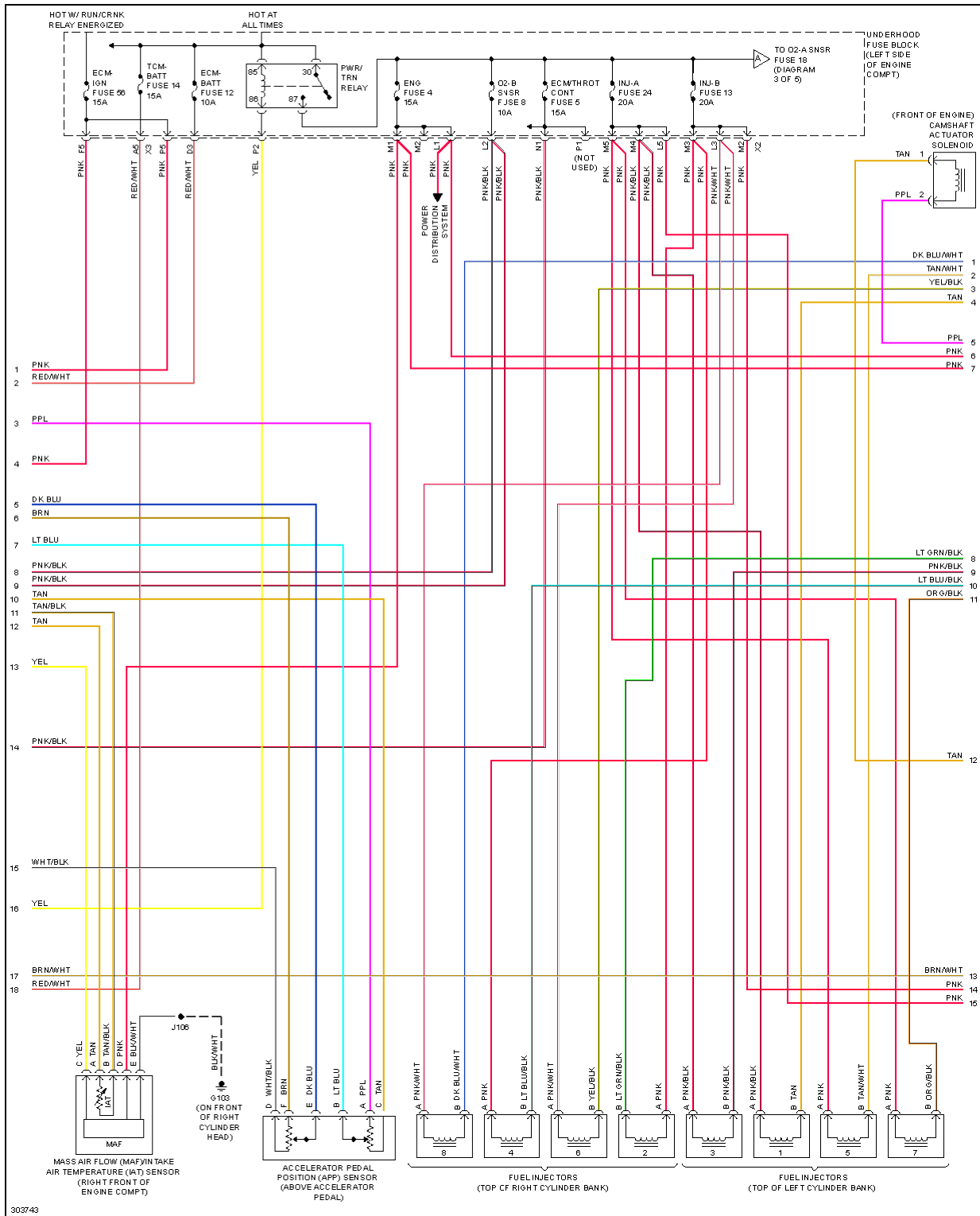
Fig. 25: 6.0L VIN K, Engine Performance Circuit (2 of 5)
