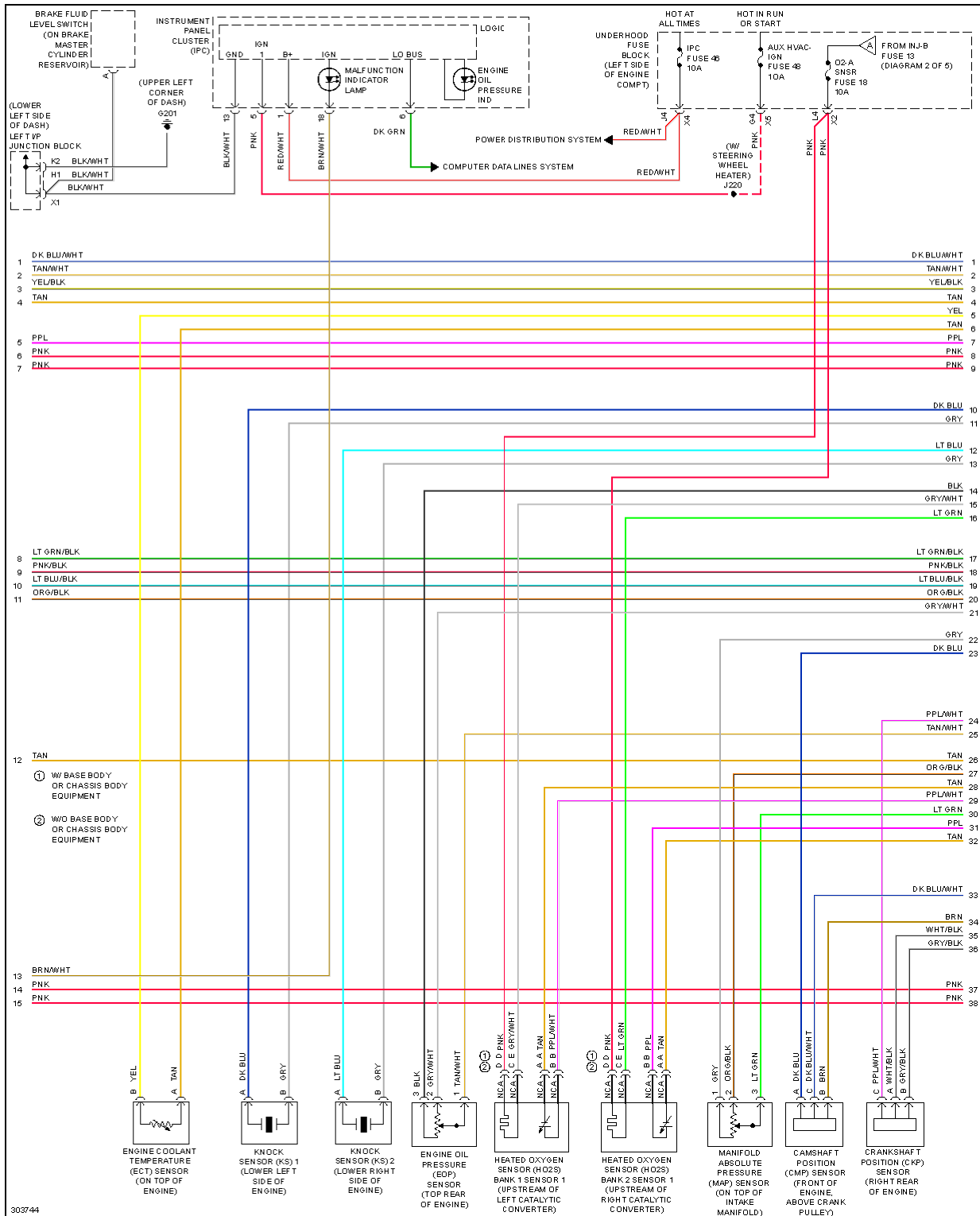
Fig. 26: 6.0L VIN K, Engine Performance Circuit (3 of 5)
