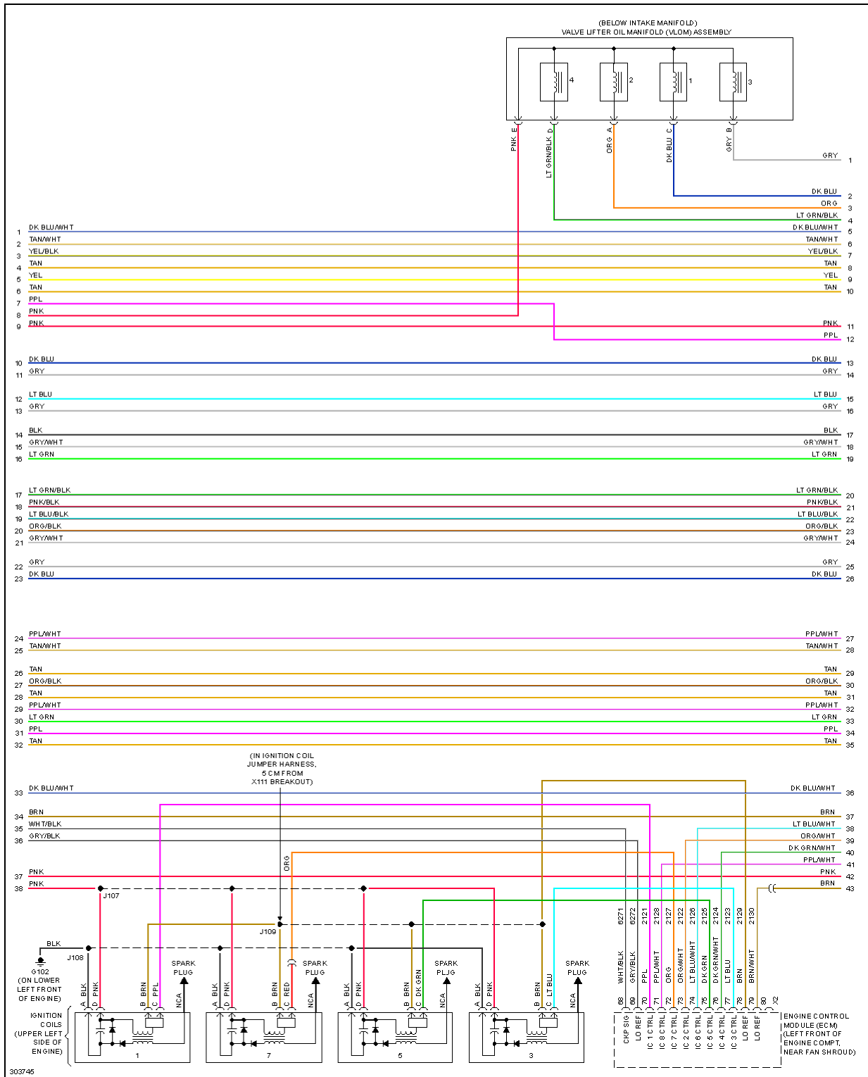
Fig. 27: 6.0L VIN K, Engine Performance Circuit (4 of 5)
