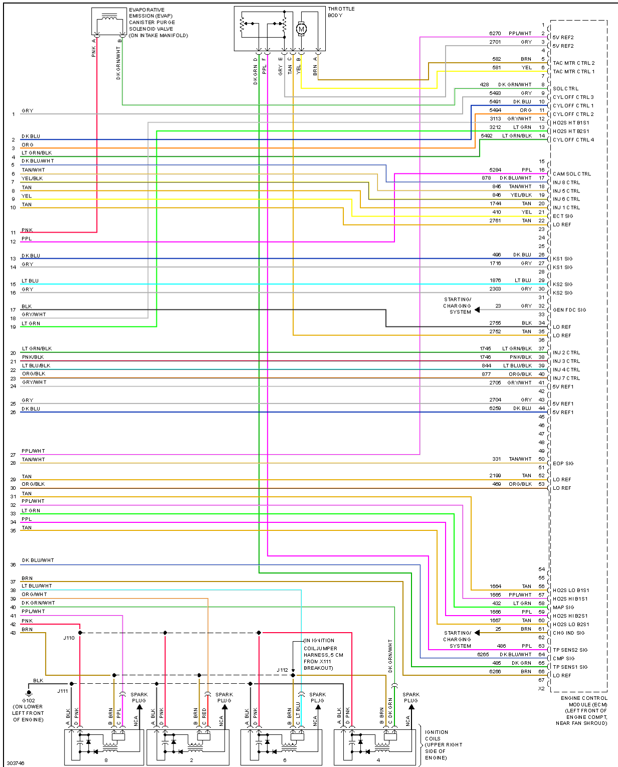
Fig. 28: 6.0L VIN K, Engine Performance Circuit (5 of 5)
