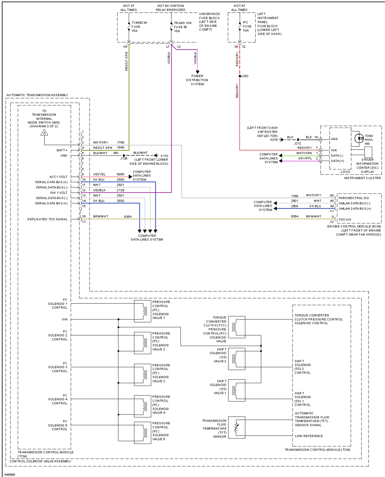
Fig. 113: A/T Circuit (1 of 2)
