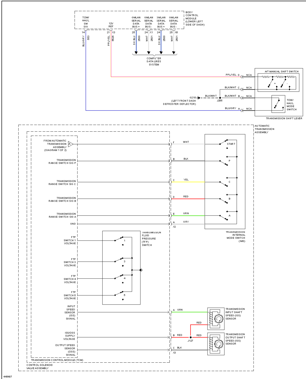
Fig. 114: A/T Circuit (2 of 2)
