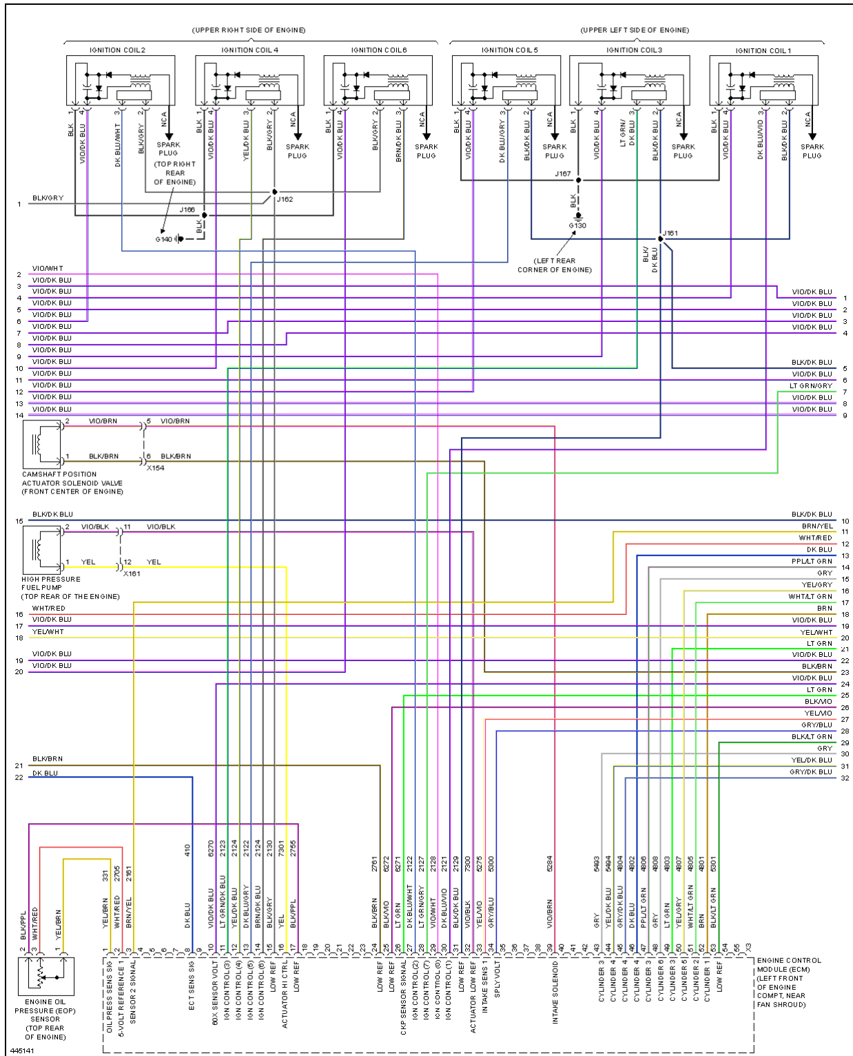
Fig. 41: 6.2L VIN J, Engine Performance Circuit (4 of 6)
