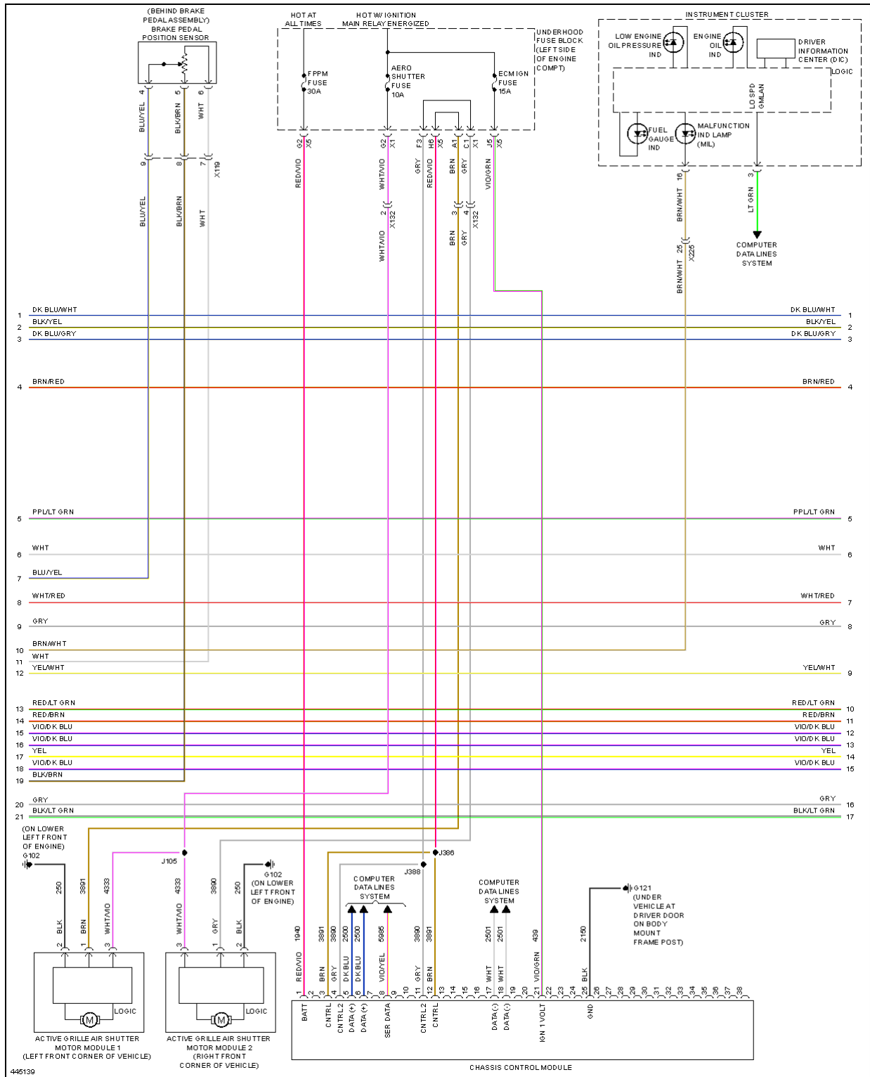
Fig. 39: 6.2L VIN J, Engine Performance Circuit (2 of 6)
