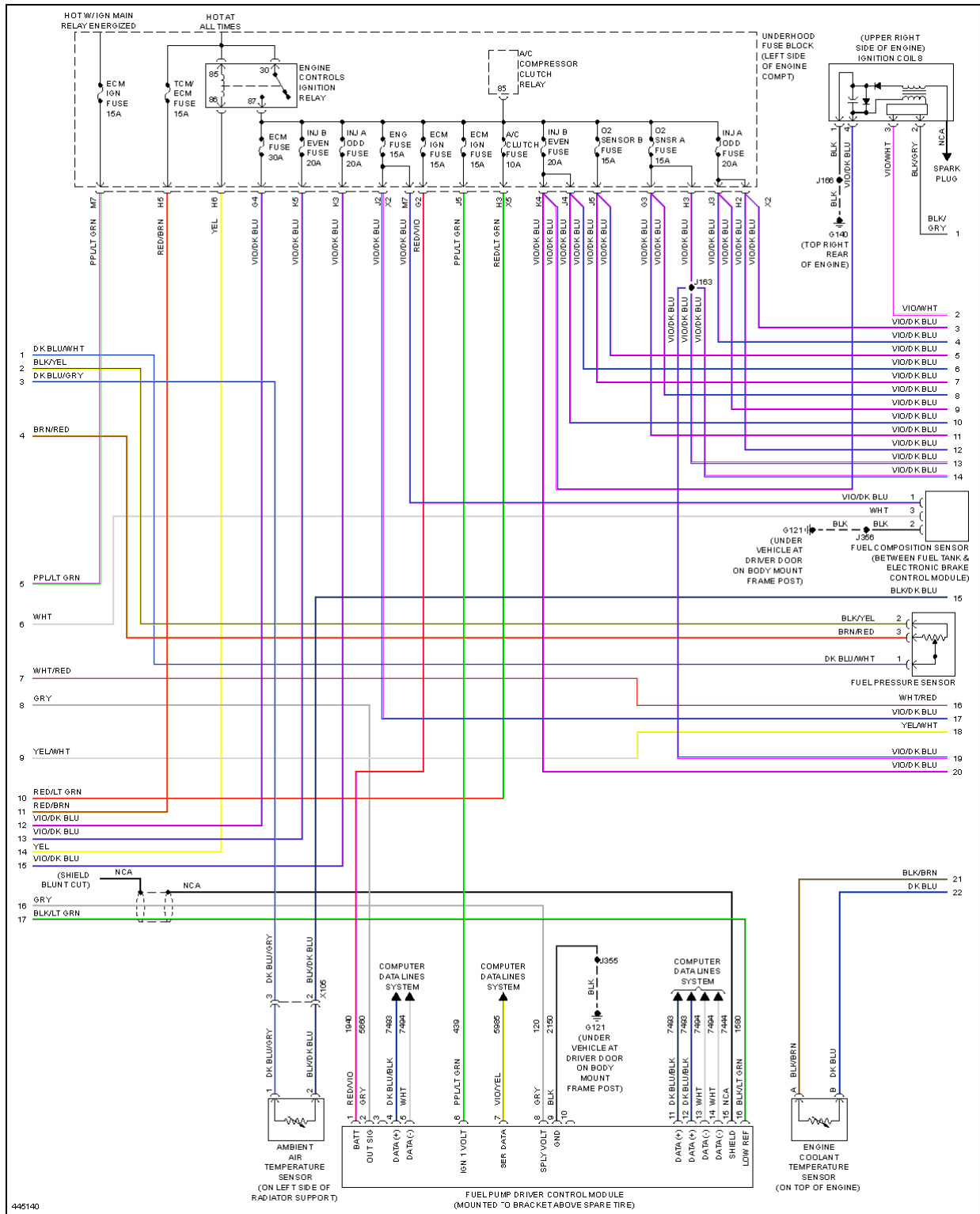
Fig. 40: 6.2L VIN J, Engine Performance Circuit (3 of 6)
