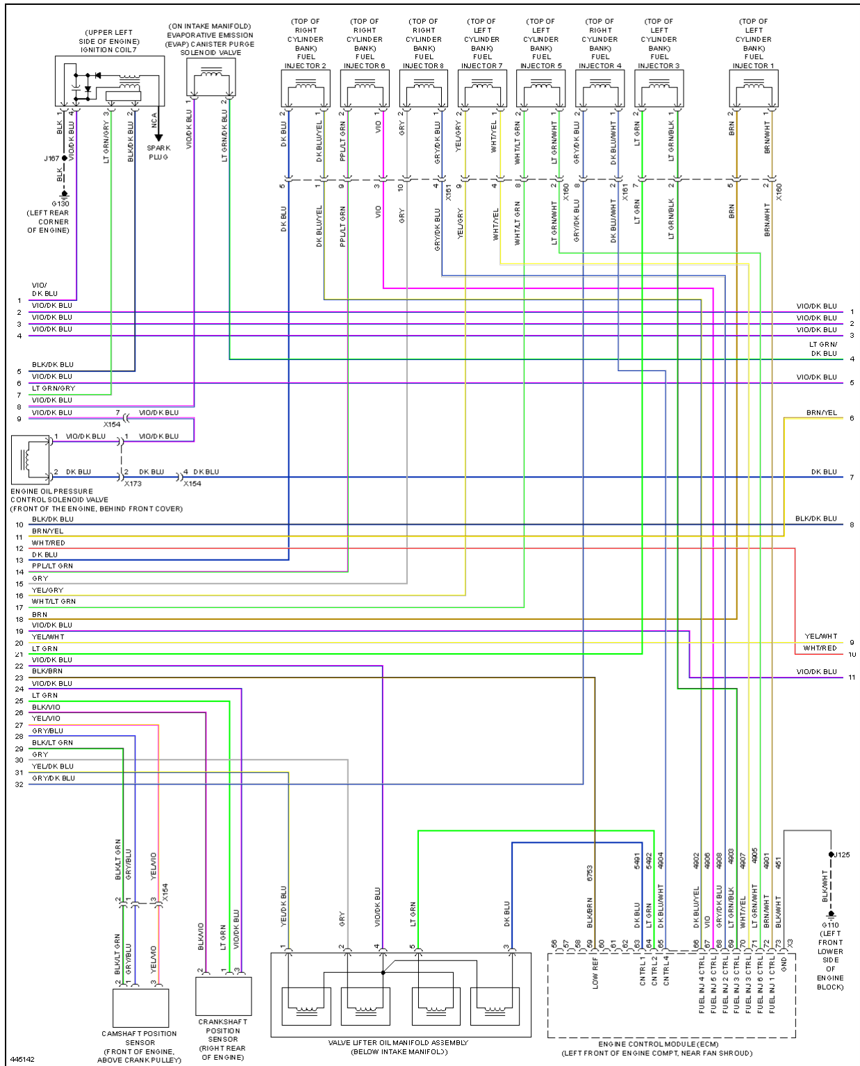
Fig. 42: 6.2L VIN J, Engine Performance Circuit (5 of 6)
