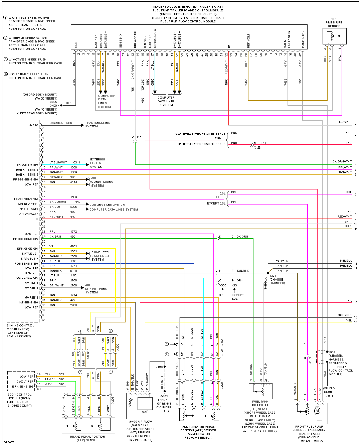
Fig. 39: 5.3L VIN 0, Engine Performance Circuit (1 of 6)
