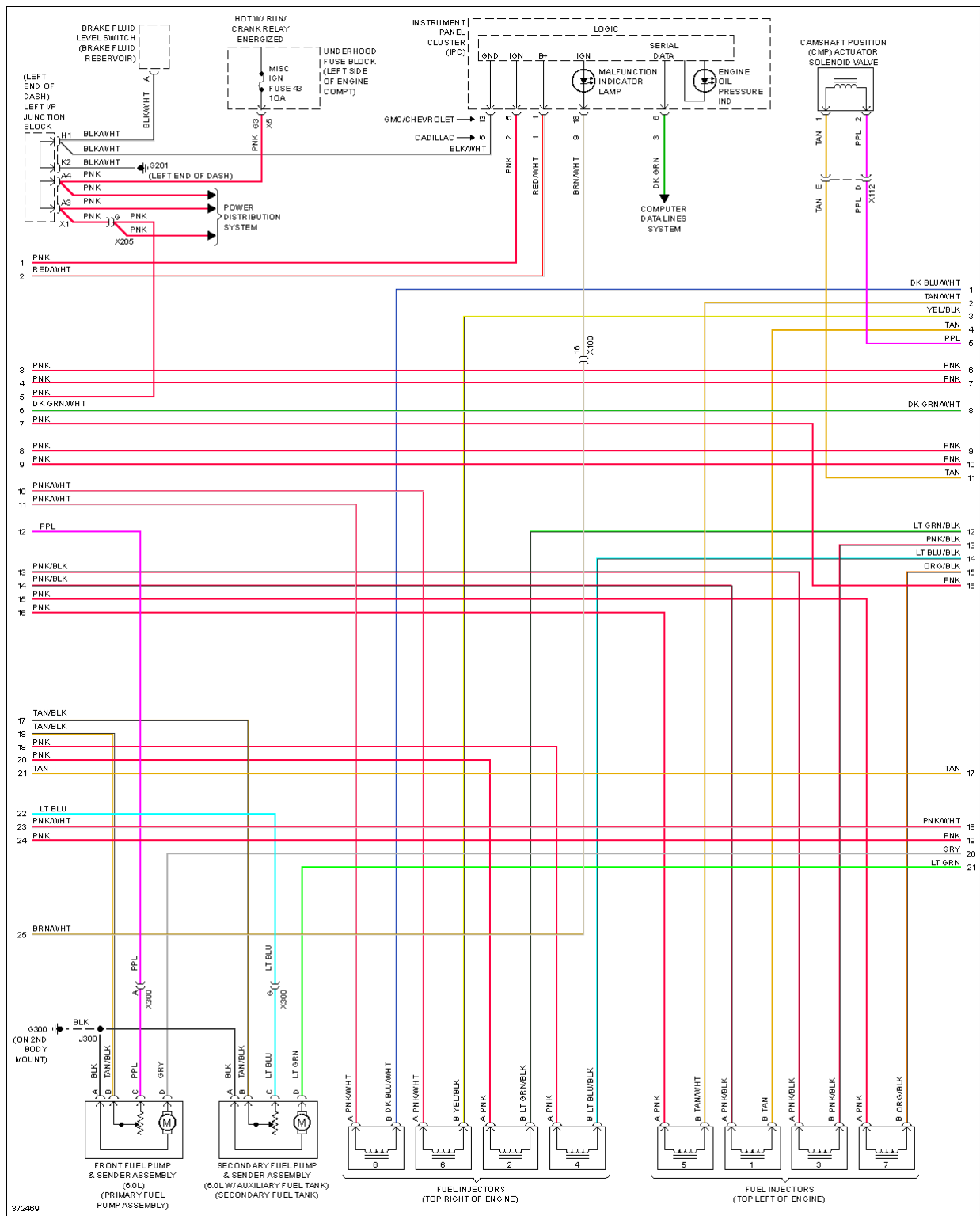
Fig. 41: 5.3L VIN 0, Engine Performance Circuit (3 of 6)
