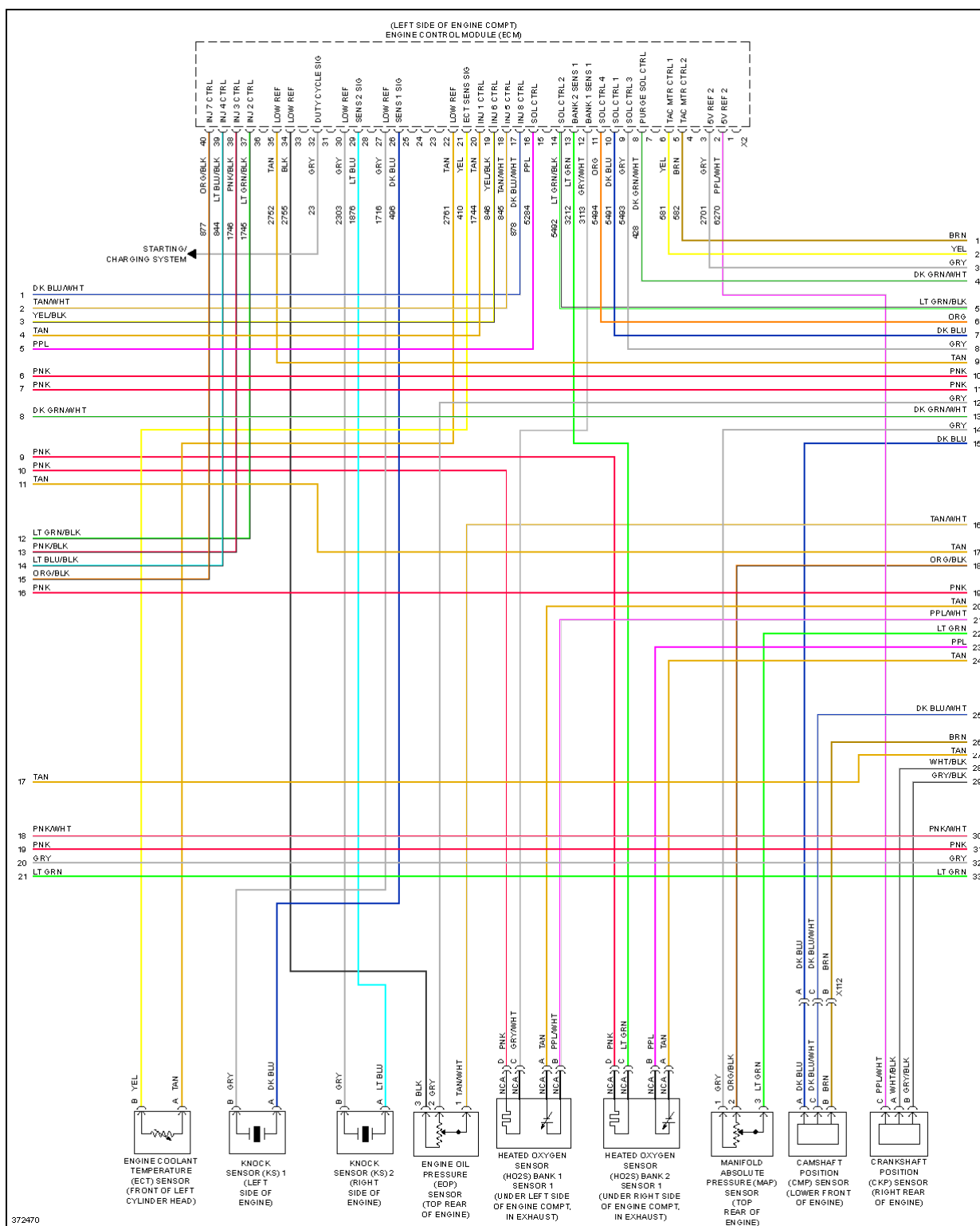
Fig. 42: 5.3L VIN 0, Engine Performance Circuit (4 of 6)
