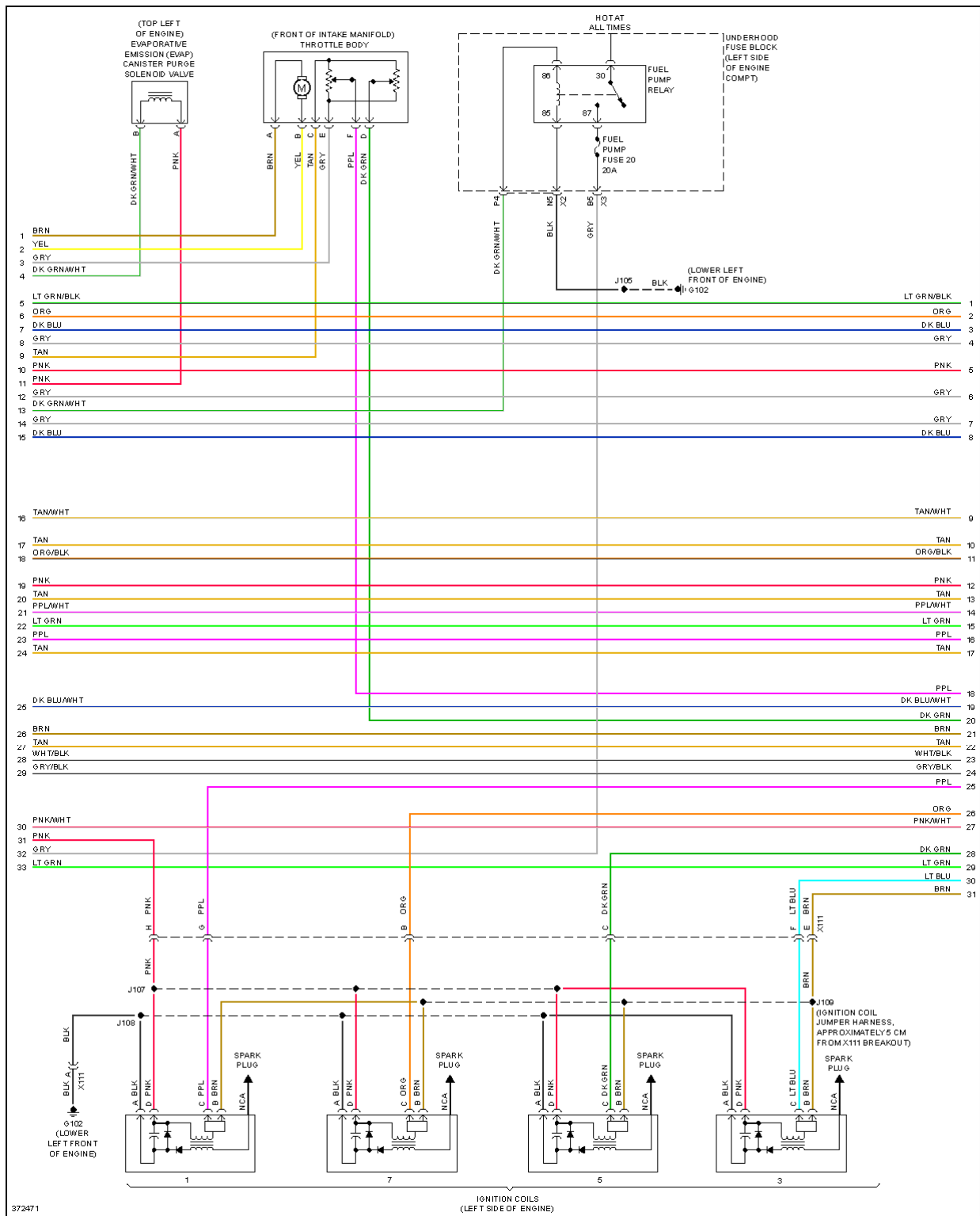
Fig. 43: 5.3L VIN 0, Engine Performance Circuit (5 of 6)
