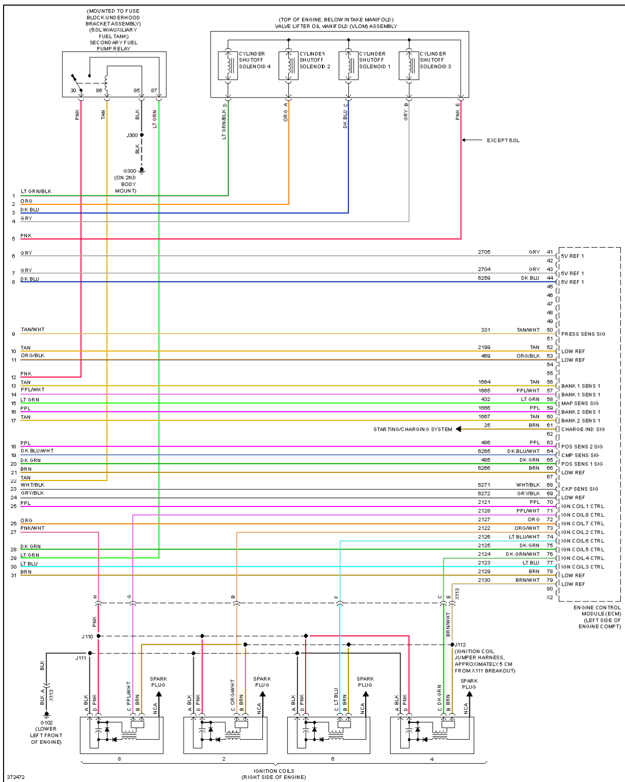
Fig. 44: 5.3L VIN 0, Engine Performance Circuit (6 of 6)
