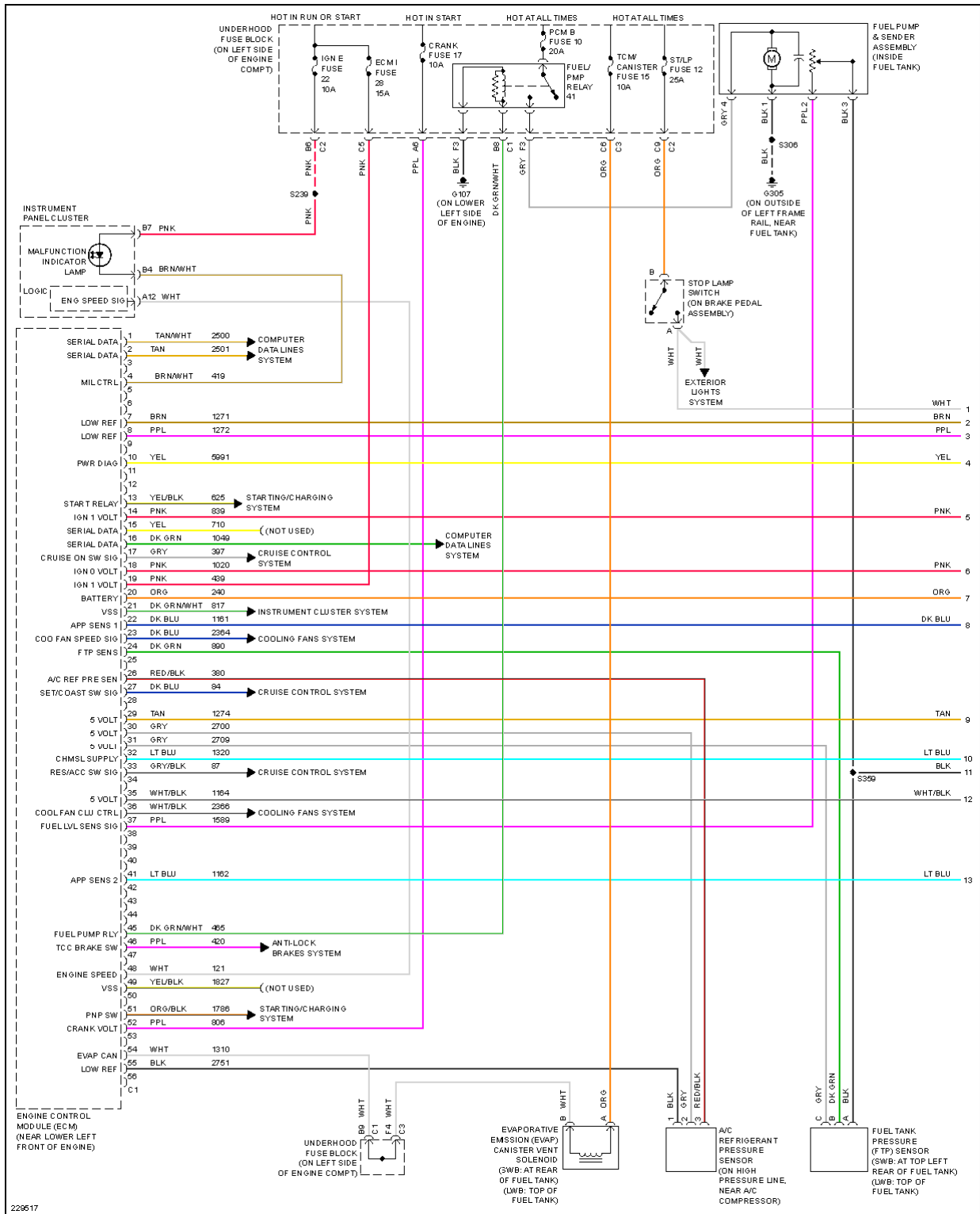
Fig. 36: 6.0L VIN H, Engine Performance Circuit (1 of 5)
