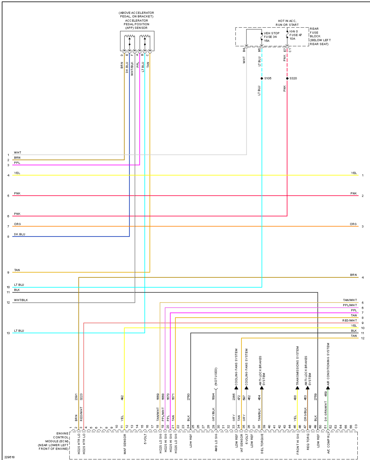
Fig. 37: 6.0L VIN H, Engine Performance Circuit (2 of 5)
