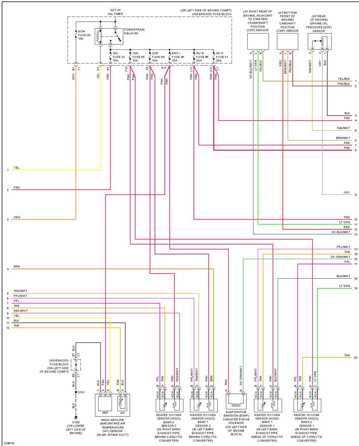
Fig. 38: 6.0L VIN H, Engine Performance Circuit (3 of 5)
