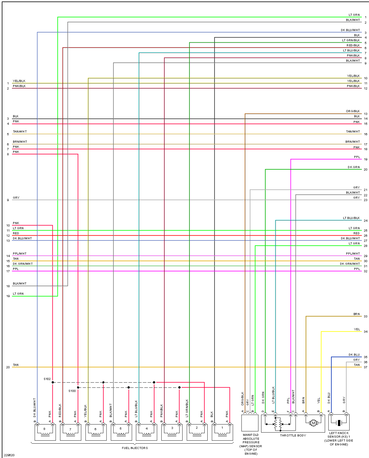
Fig. 39: 6.0L VIN H, Engine Performance Circuit (4 of 5)
