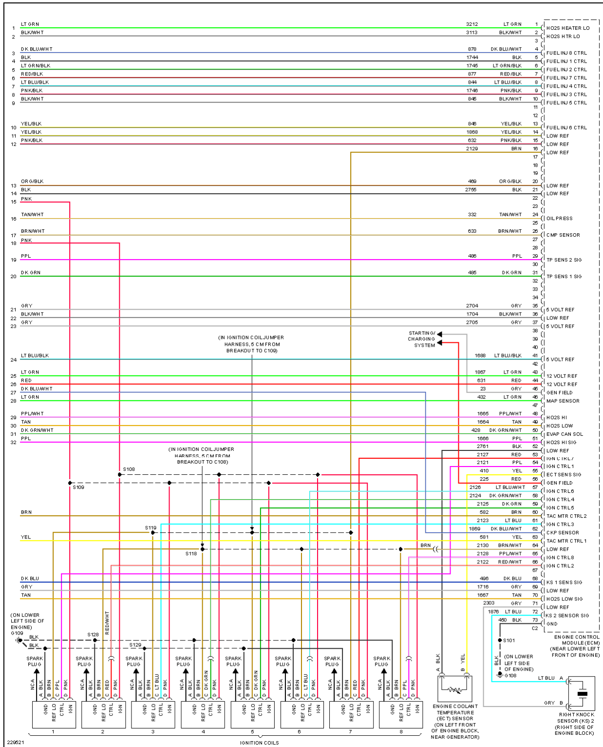
Fig. 40: 6.0L VIN H, Engine Performance Circuit (5 of 5)
