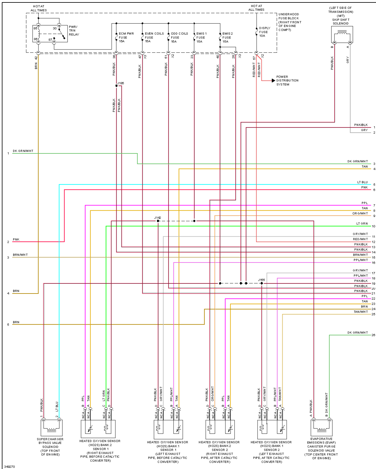
Fig. 37: 6.2L VIN P, Engine Performance Circuit (2 of 6)
