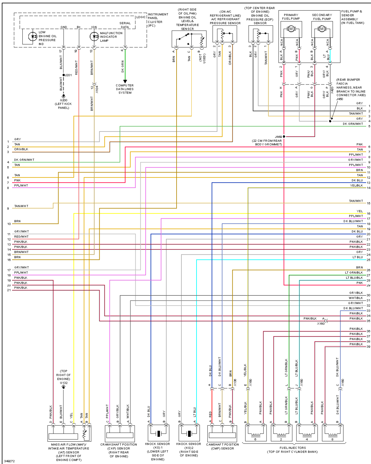
Fig. 39: 6.2L VIN P, Engine Performance Circuit (4 of 6)
