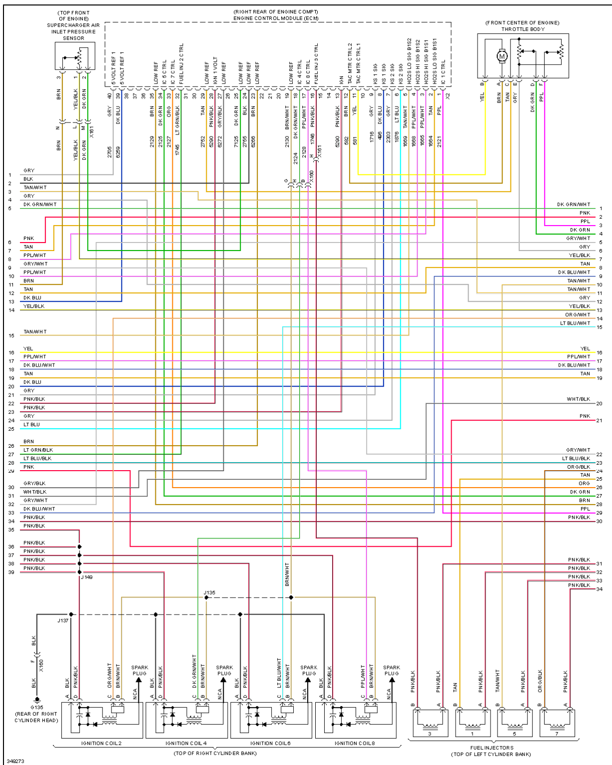
Fig. 40: 6.2L VIN P, Engine Performance Circuit (5 of 6)
